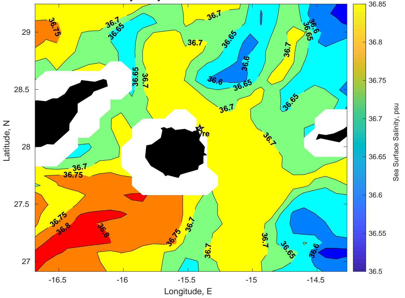
Surface Salinity for Gyre at 20-Feb-2025 00:00:00
