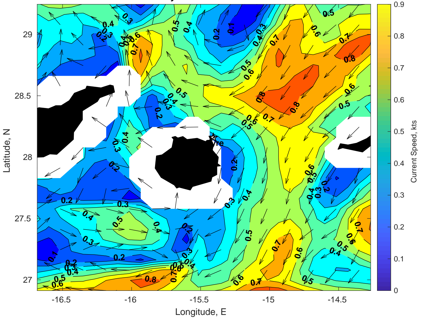
Surface Currents for Gyre at 20-Feb-2025 00:00:00
