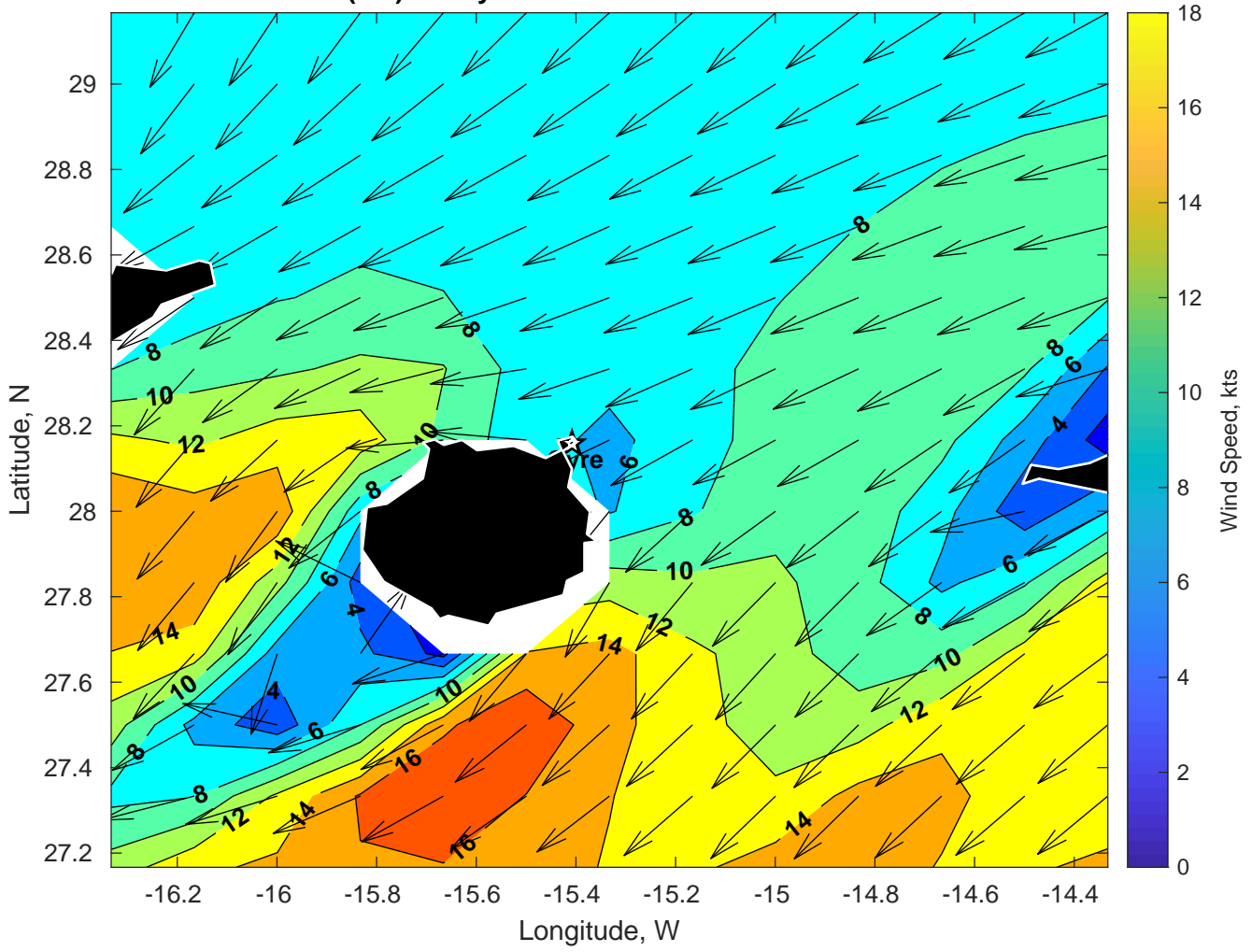
Winds (kts) for Gyre at 21-Feb-2025 09:00:00
