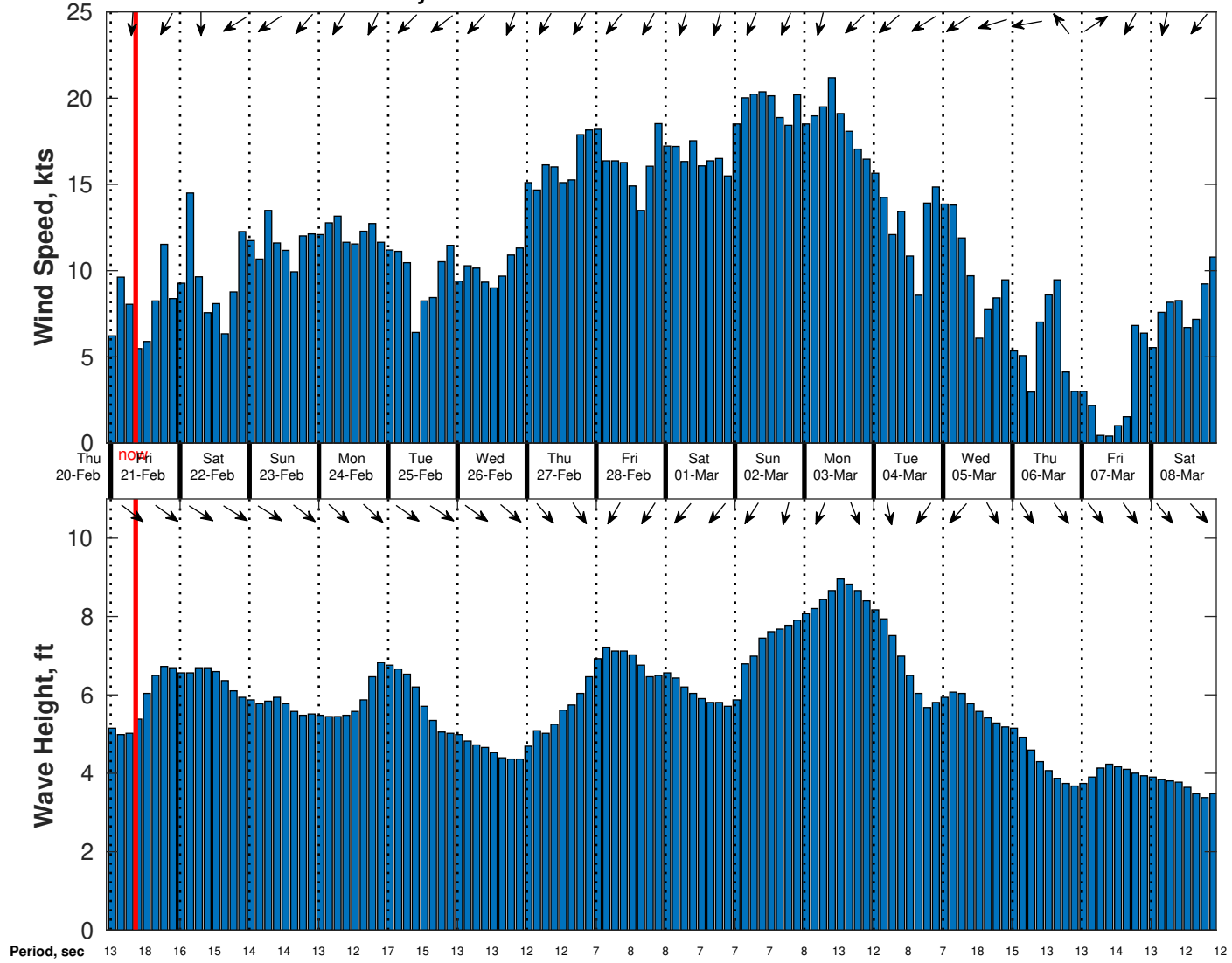
Wind & Wave Forecast for Gyre from 20-Feb-2025 23:00:00 to 08-Mar-2025 23:00:00
