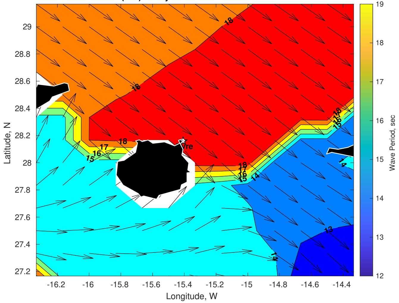
Wave Period (sec) for Gyre at 21-Feb-2025 09:00:00
