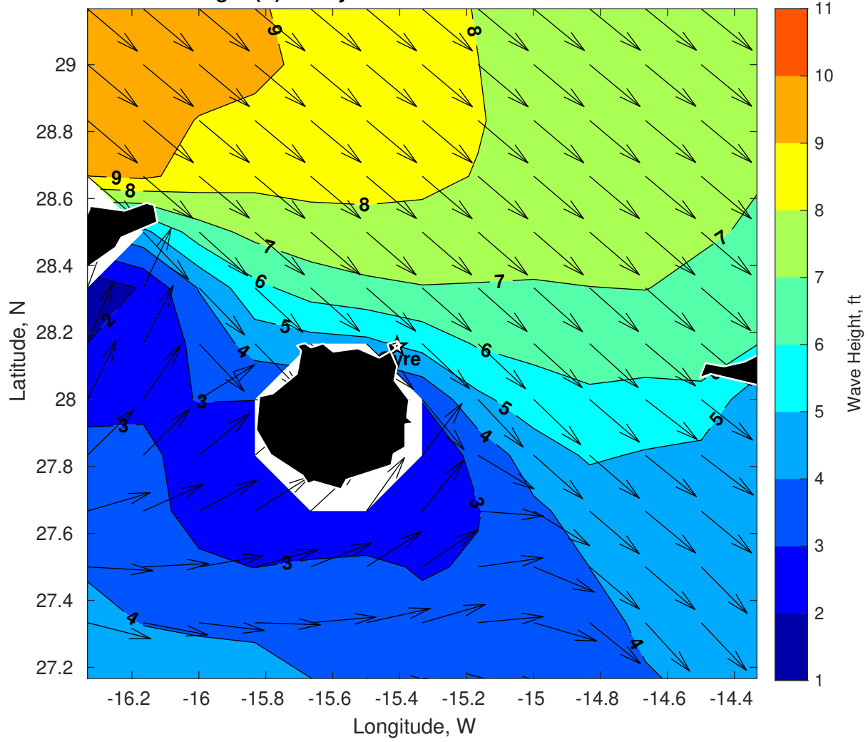
Wave Height (ft) for Gyre at 21-Feb-2025 09:00:00
