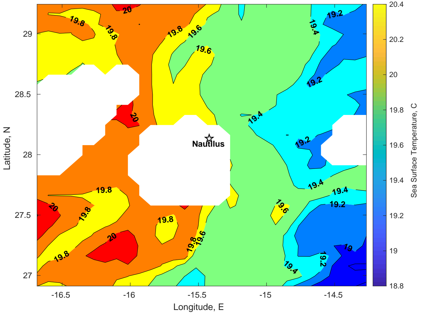
SST for Nautilus at 20-Feb-2025 00:00:00
