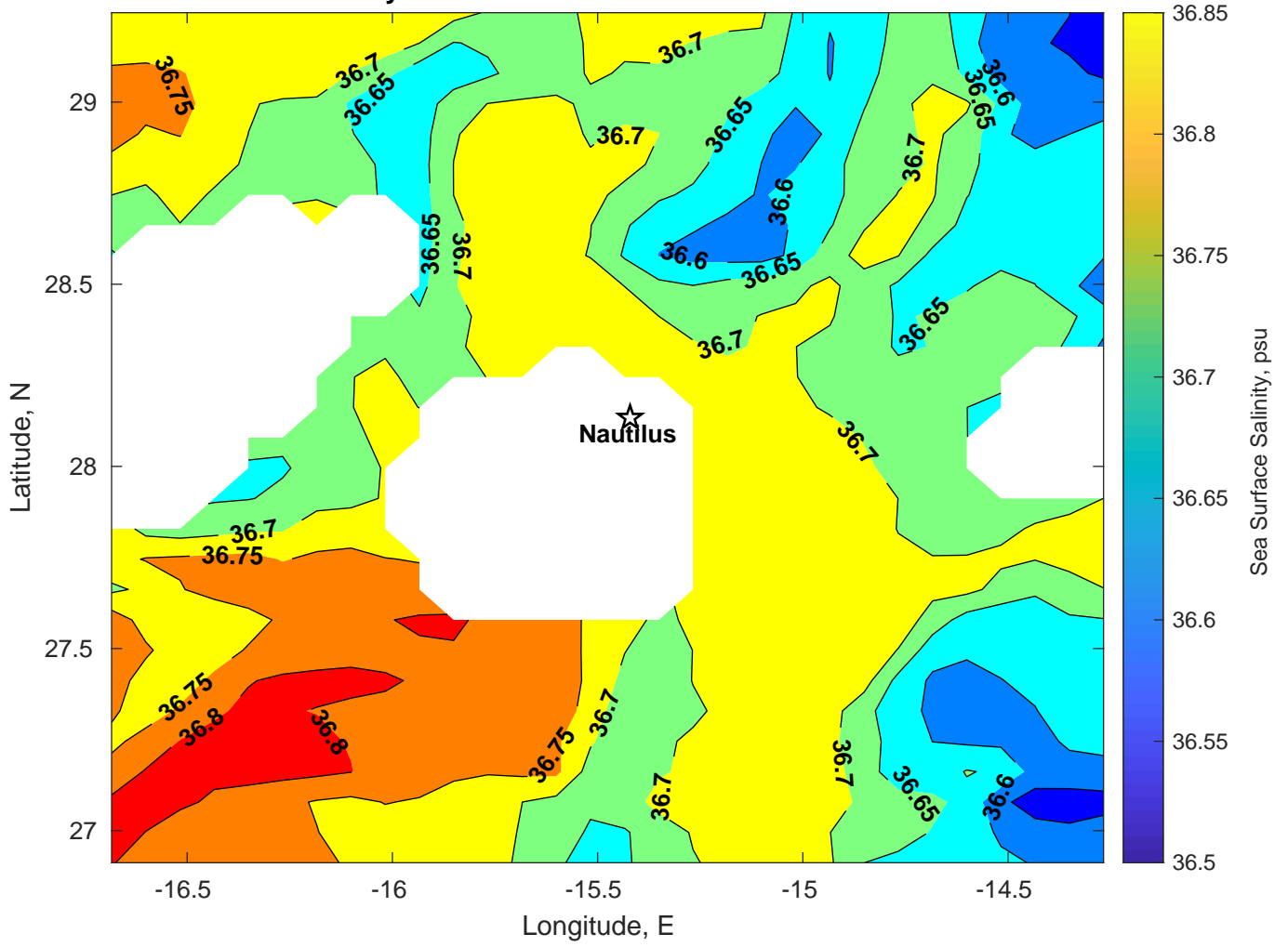
Surface Salinity for Nautilus at 20-Feb-2025 00:00:00
