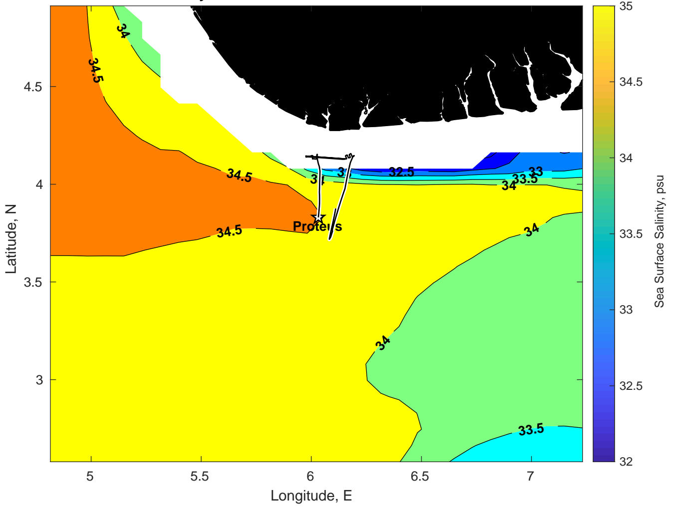
Surface Salinity for Proteus at 20-Feb-2025 00:00:00
