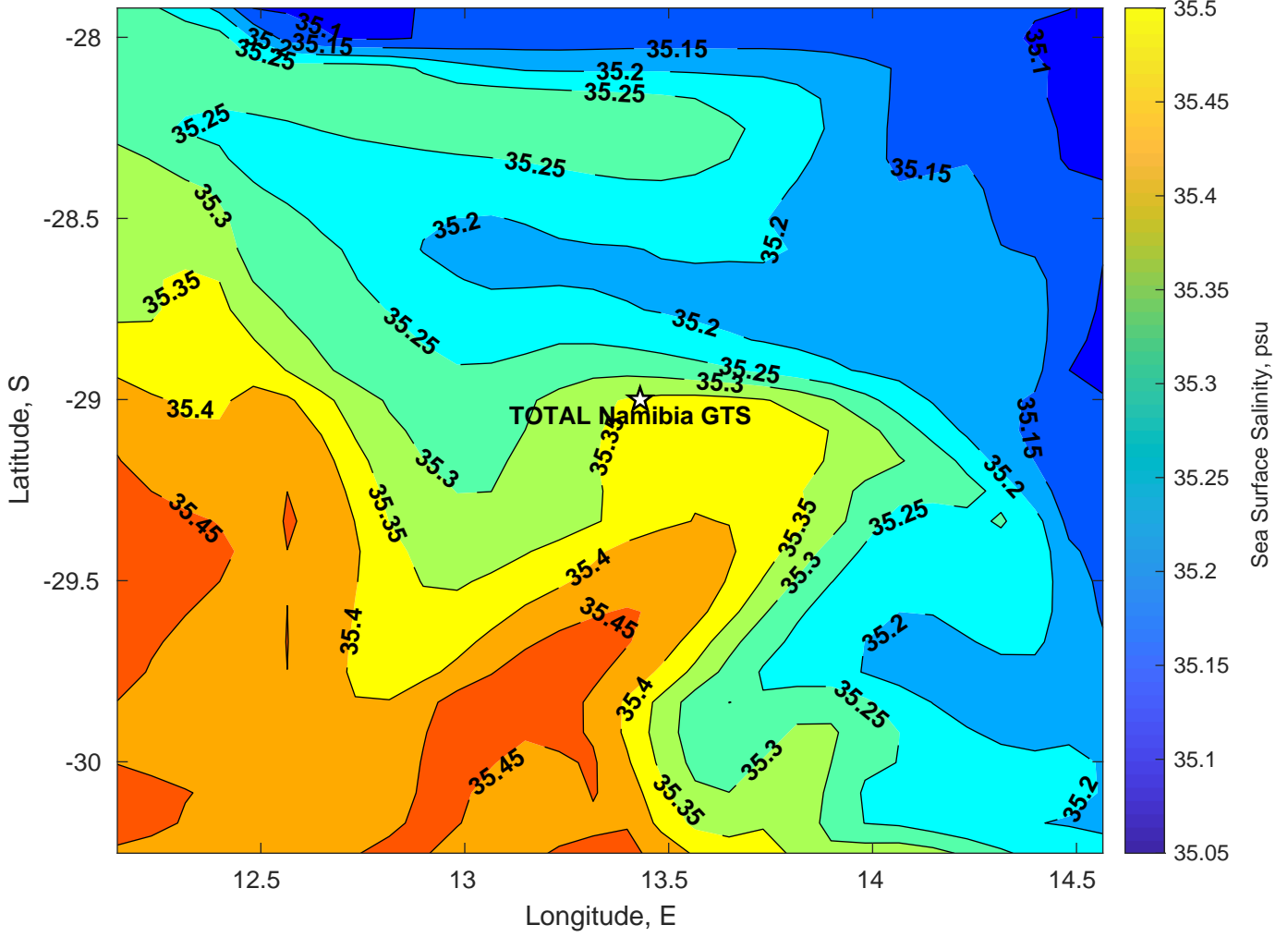
Surface Salinity for TOTAL Namibia GTS at 19-Feb-2025 00:00:00
