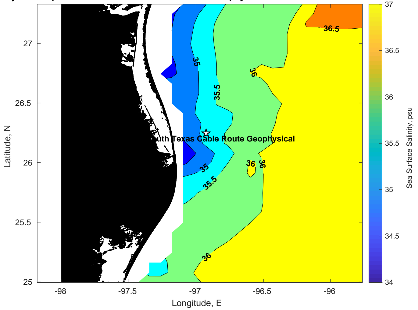
Surface Salinity for Tampnet P2378 South Texas Cable Route Geophysical at 19-Feb-2025 00:00:00
