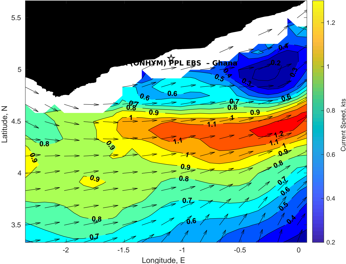
Surface Currents for CSA (ONHYM) PPL EBS - Ghana at 21-Feb-2025 00:00:00
