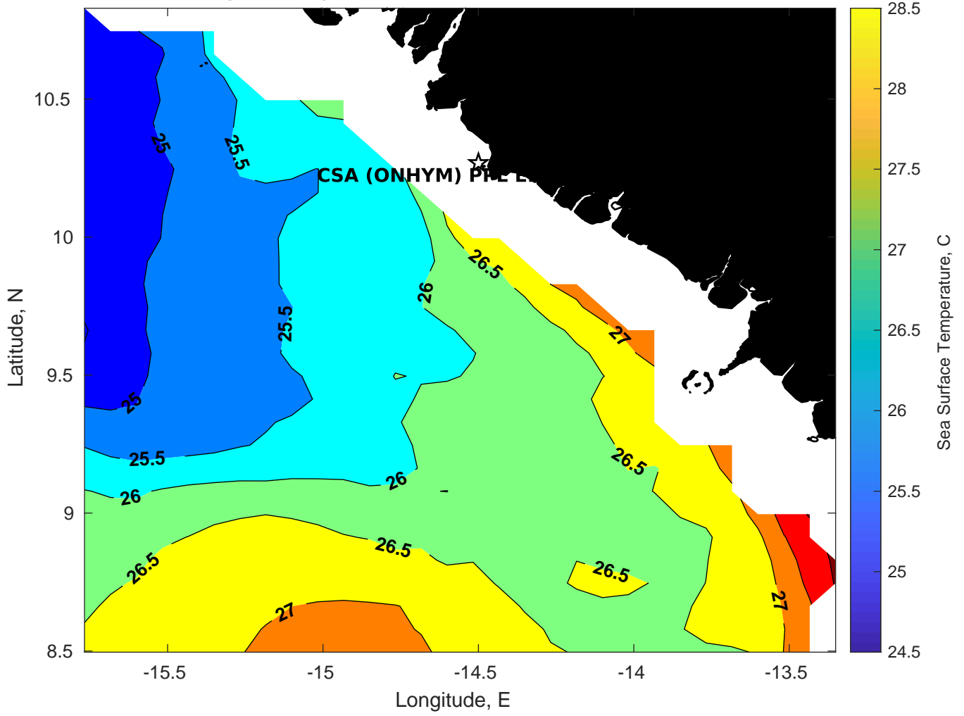
SST for CSA (ONHYM) PPL EBS - Guinea at 21-Feb-2025 00:00:00
