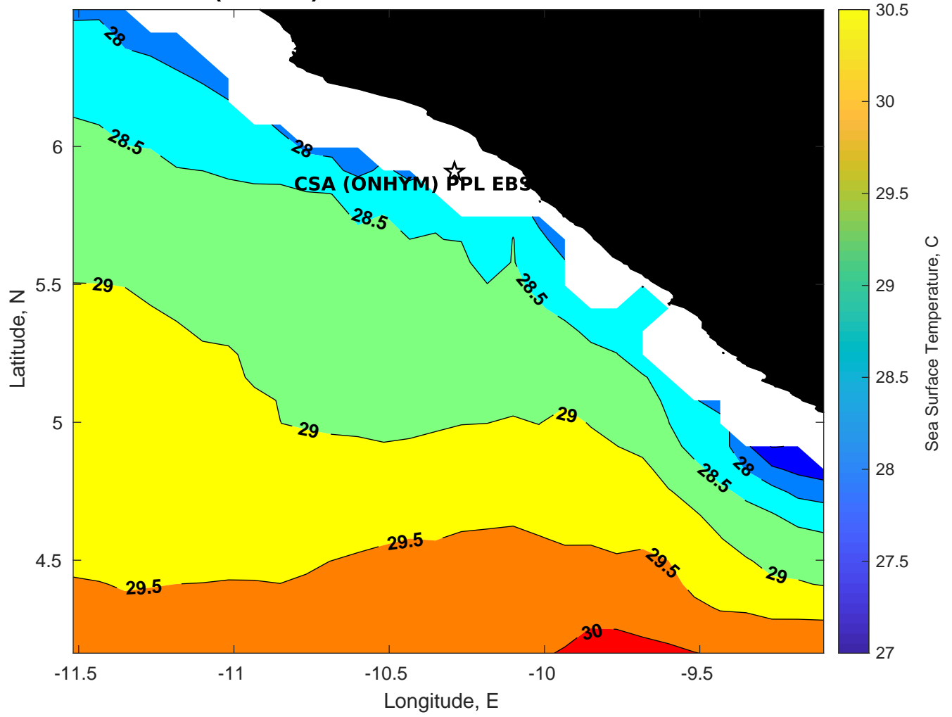
SST for CSA (ONHYM) PPL EBS - Liberia at 21-Feb-2025 00:00:00
