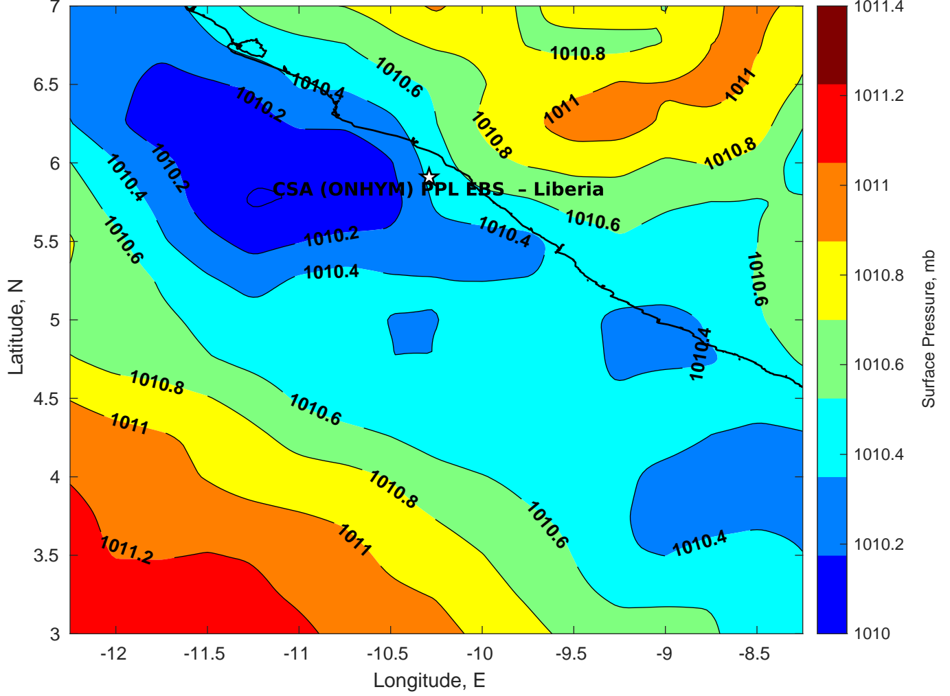
Surface Pressure (mb) for CSA (ONHYM) PPL EBS - Liberia at 22-Feb-2025 00:00:00
