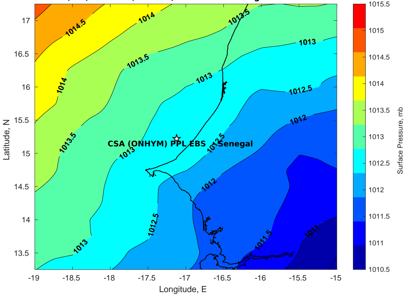
Surface Pressure (mb) for CSA (ONHYM) PPL EBS - Senegal at 22-Feb-2025 00:00:00
