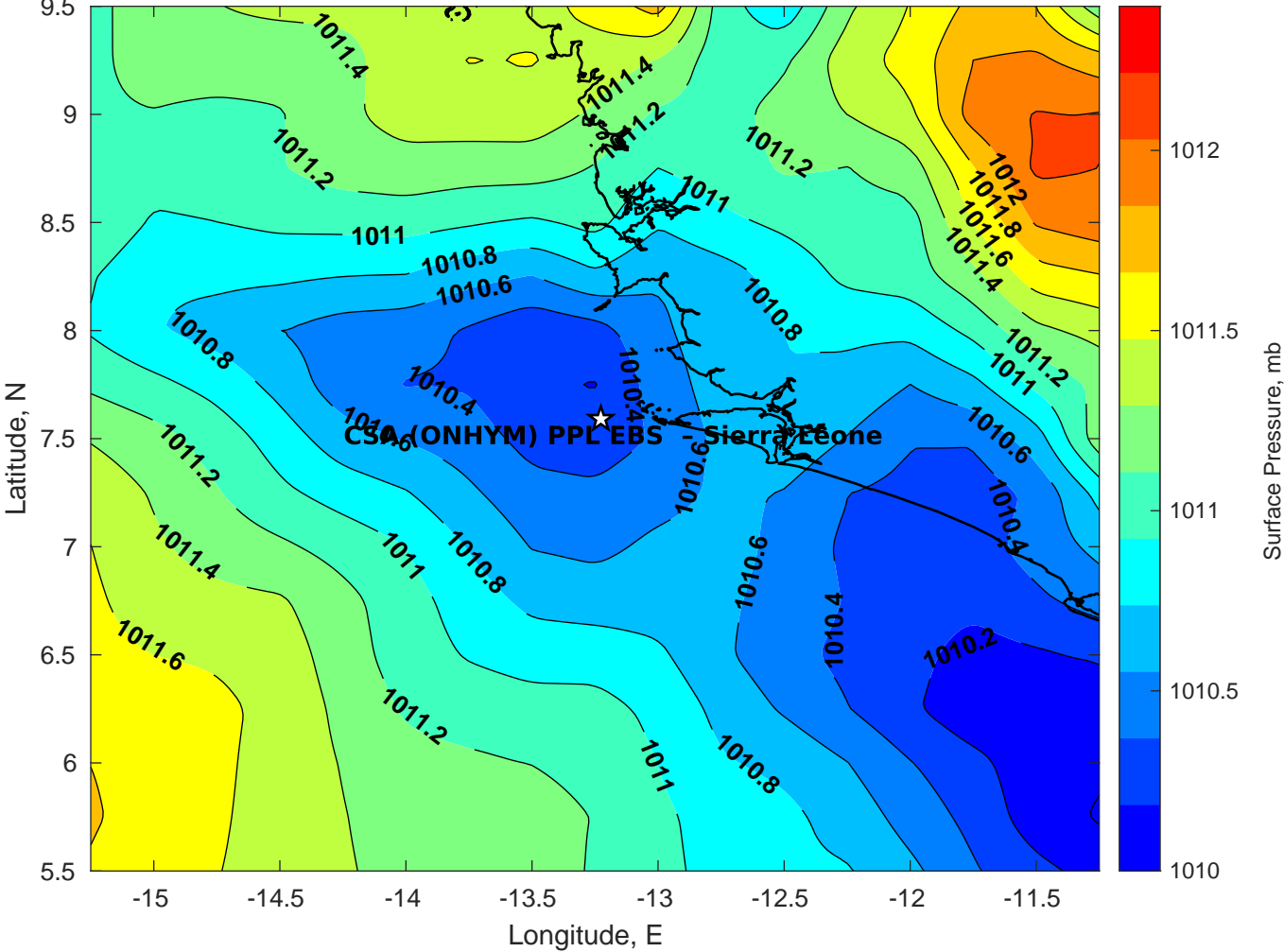
Surface Pressure (mb) for CSA (ONHYM) PPL EBS - Sierra Leone at 22-Feb-2025 00:00:00
