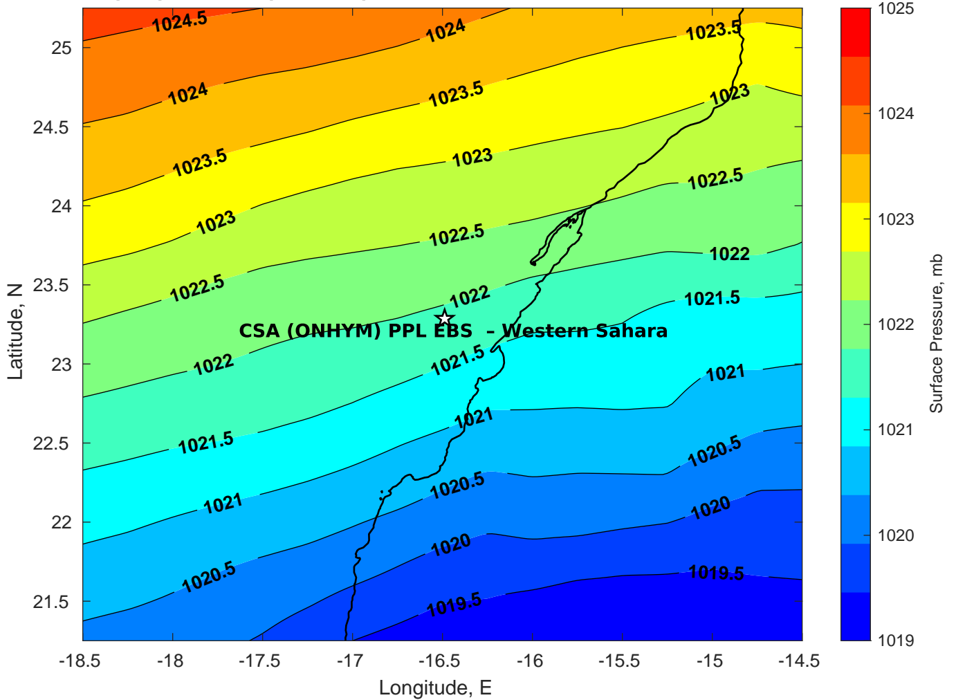
Surface Pressure (mb) for CSA (ONHYM) PPL EBS - Western Sahara at 24-Feb-2025 00:00:00
