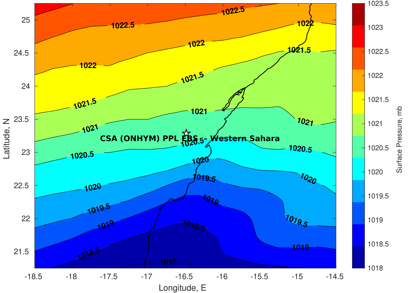
Surface Pressure (mb) for CSA (ONHYM) PPL EBS - Western Sahara at 22-Feb-2025 00:00:00
