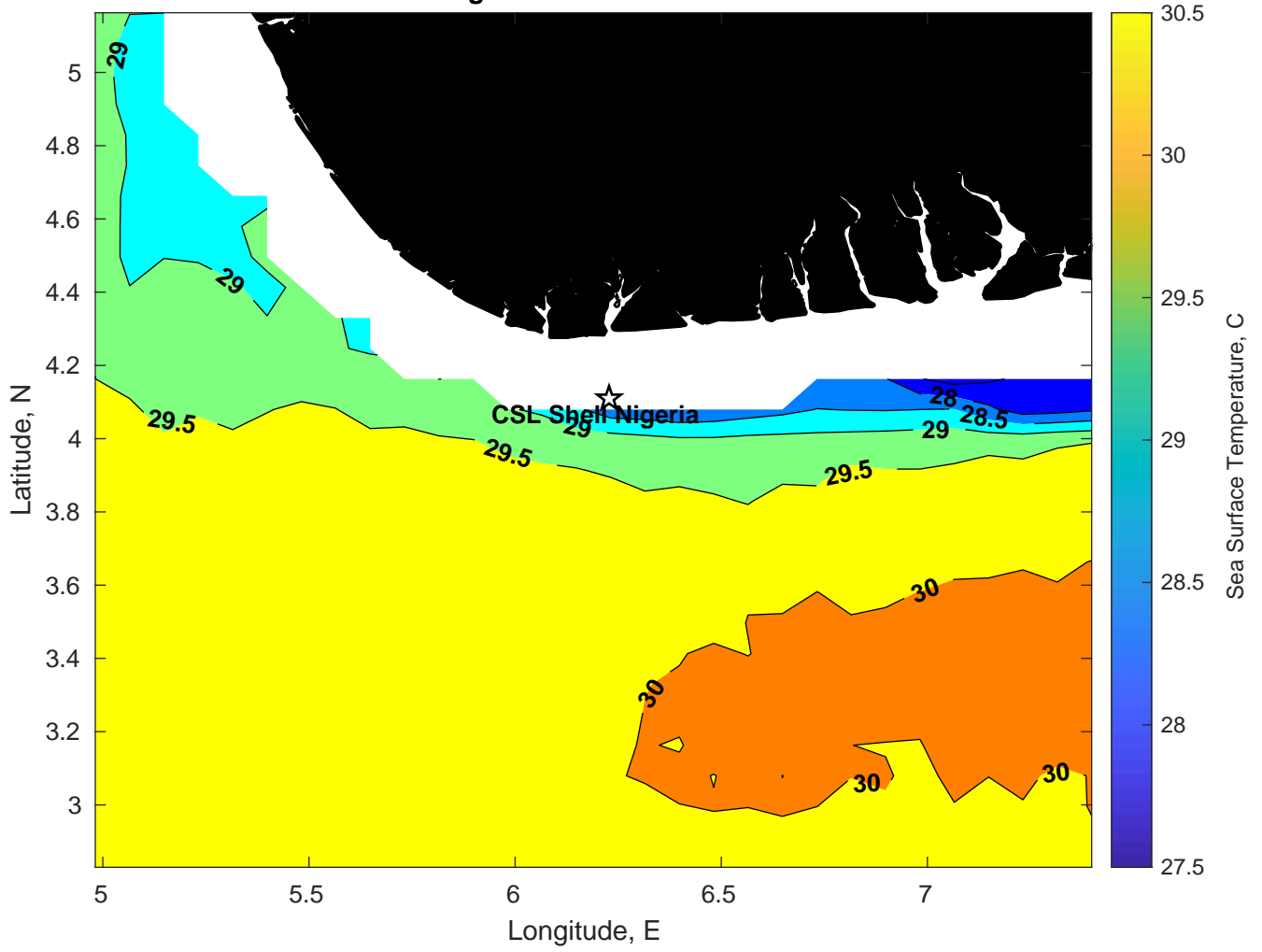
SST for CSL Shell Nigeria at 21-Feb-2025 00:00:00
