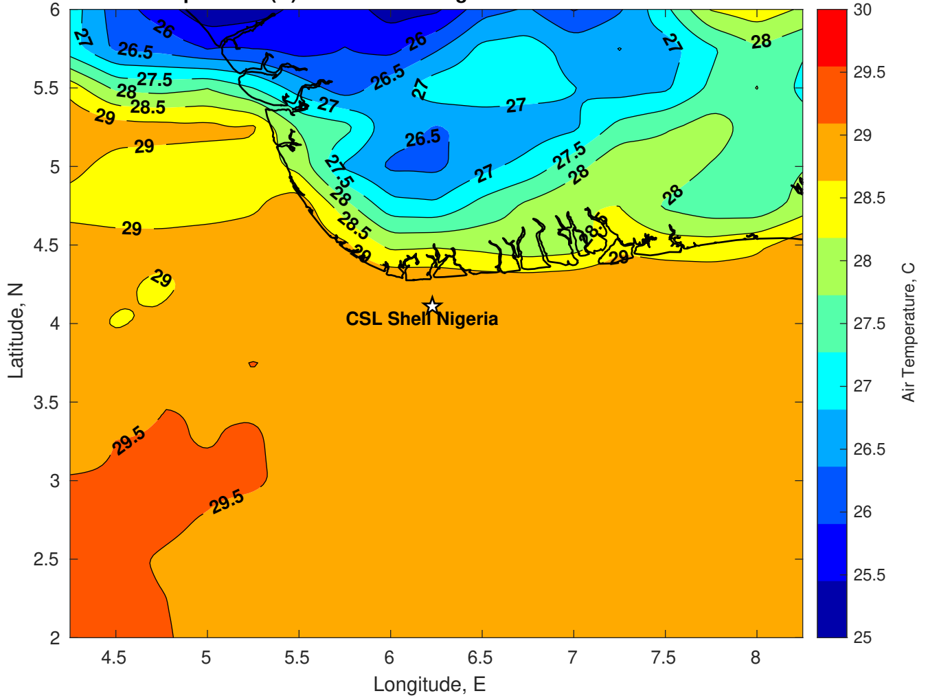
Air Temperature (C) for CSL Shell Nigeria at 22-Feb-2025
