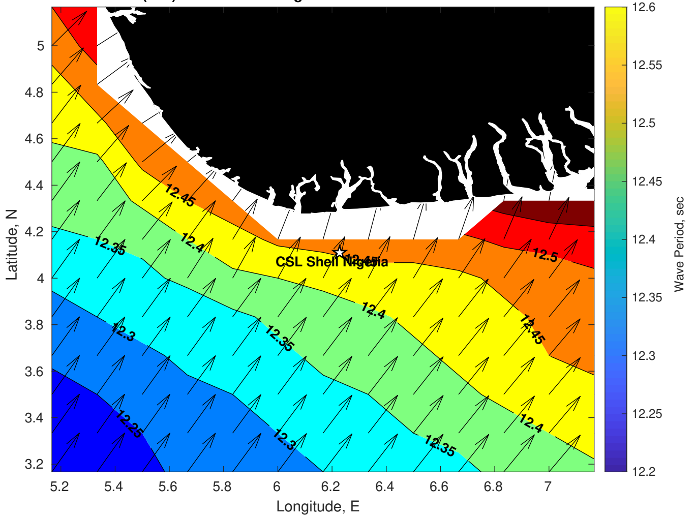
Wave Period (sec) for CSL Shell Nigeria at 22-Feb-2025 09:00:00
