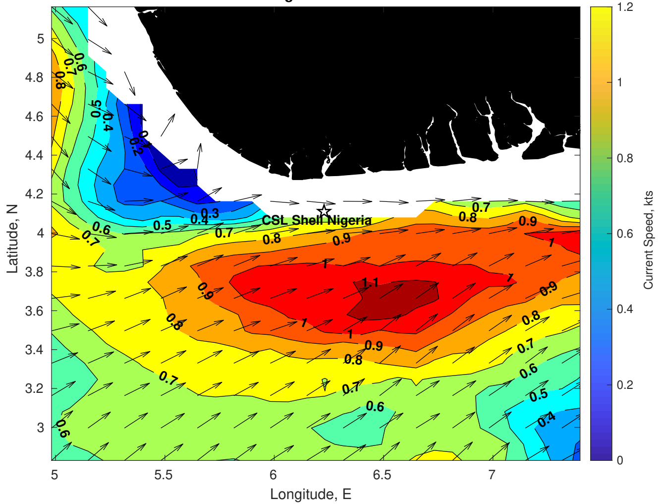
Surface Currents for CSL Shell Nigeria at 21-Feb-2025 00:00:00
