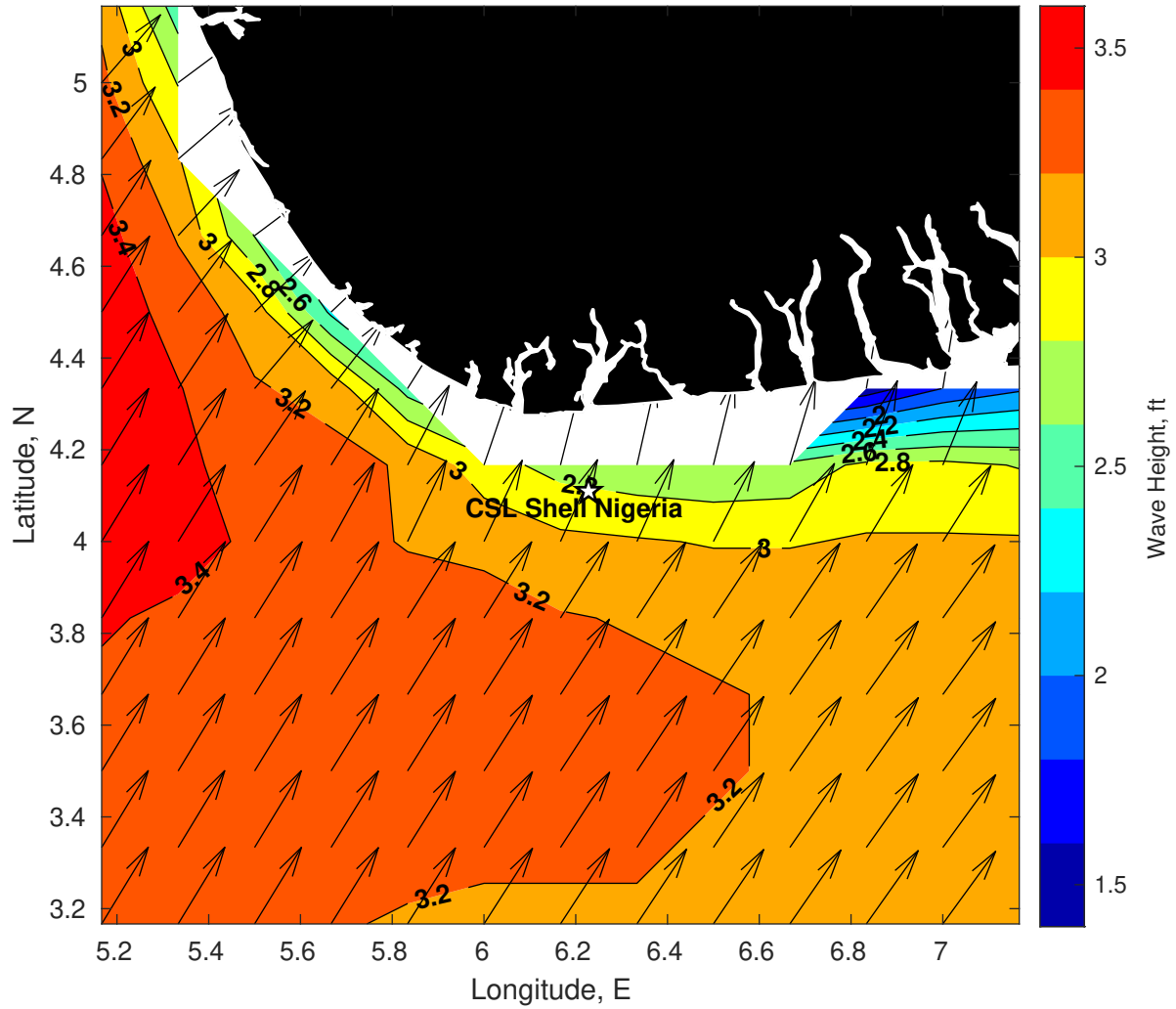
Wave Height (ft) for CSL Shell Nigeria at 22-Feb-2025 09:00:00
