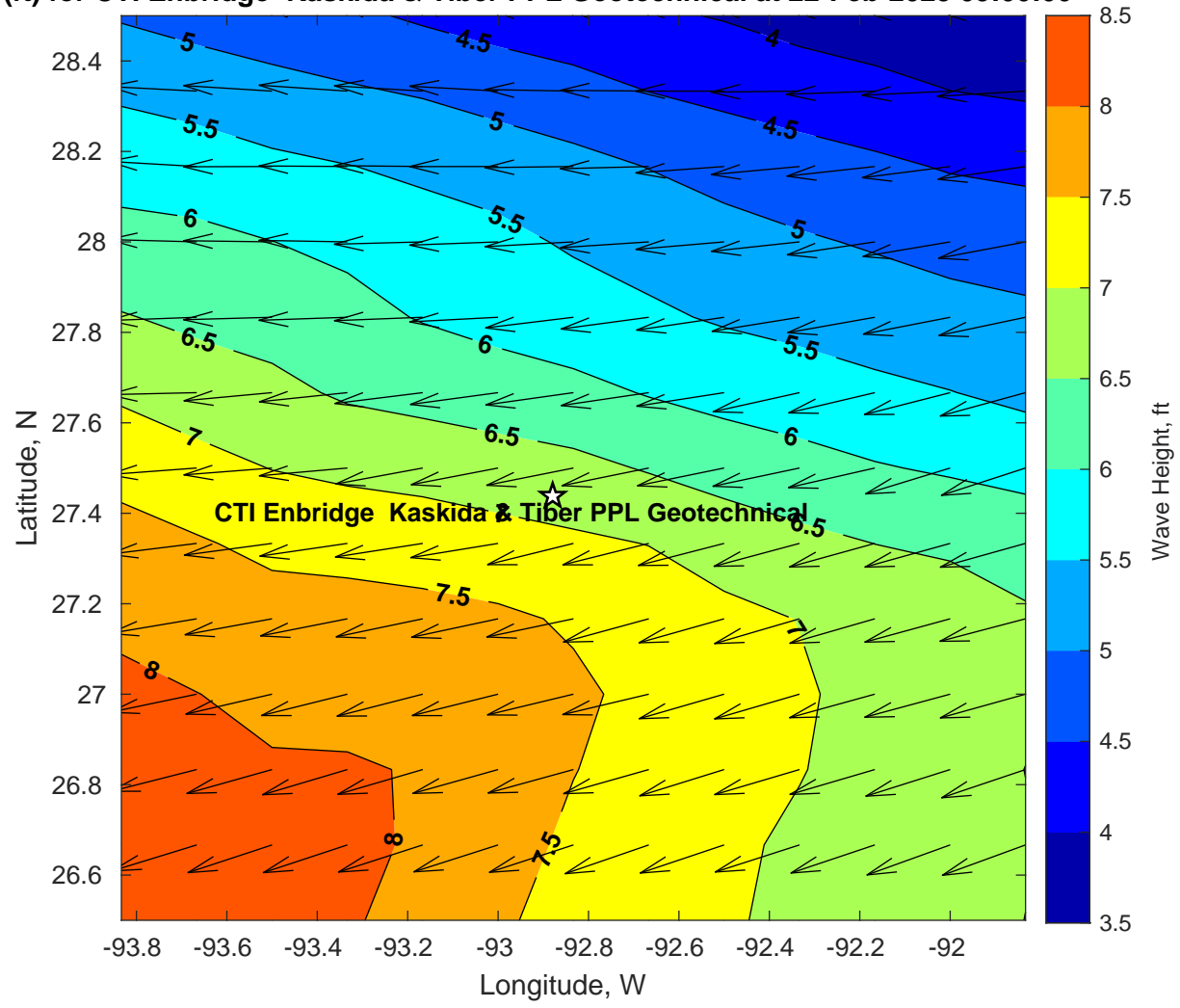
Wave Height (ft) for CTI Enbridge Kaskida & Tiber PPL Geotechnical at 22-Feb-2025 09:00:00
