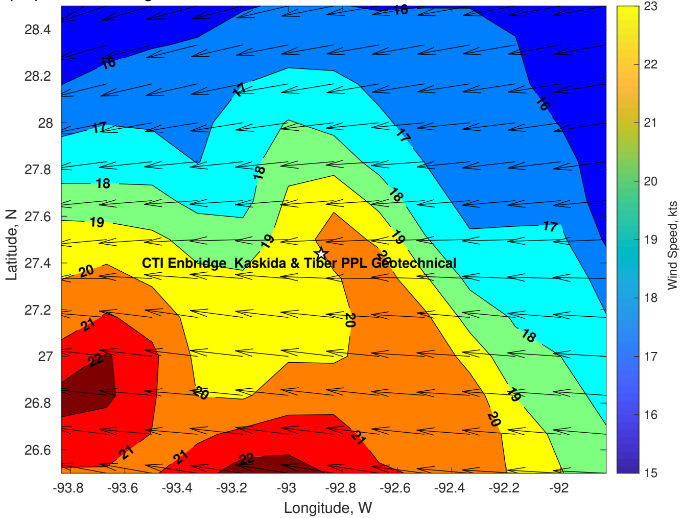
Winds (kts) for CTI Enbridge Kaskida & Tiber PPL Geotechnical at 22-Feb-2025 09:00:00
