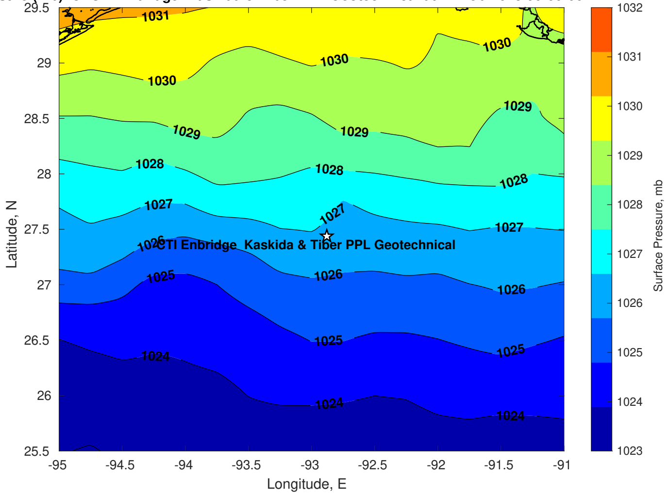
Surface Pressure (mb) for CTI Enbridge Kaskida & Tiber PPL Geotechnical at 22-Feb-2025 00:00:00
