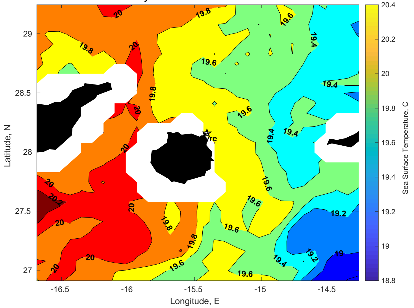
SST for Gyre at 21-Feb-2025 00:00:00
