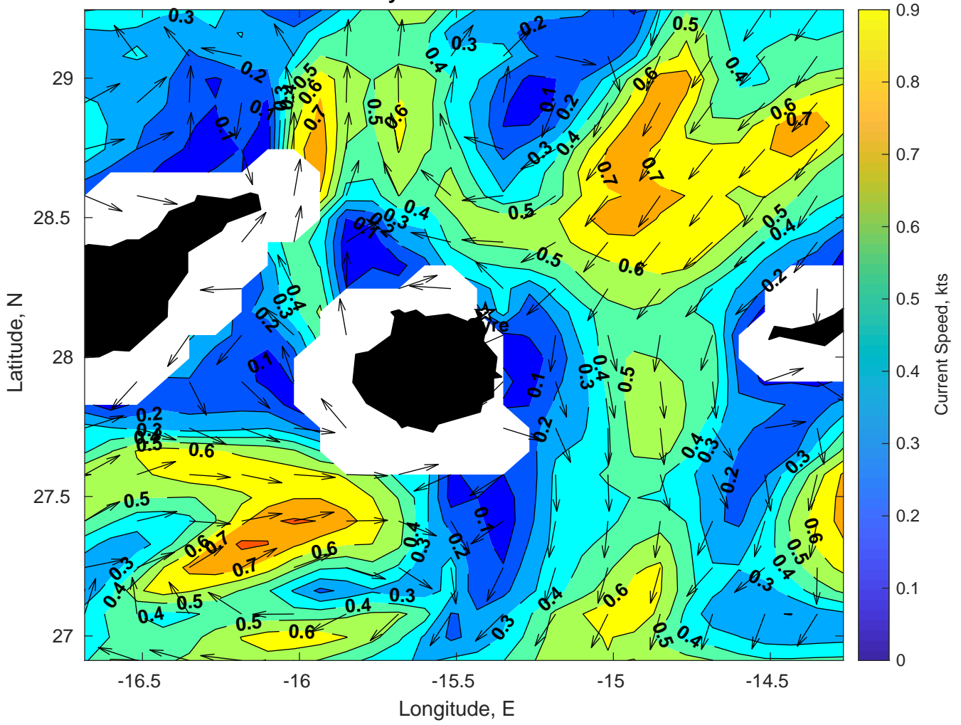
Surface Currents for Gyre at 21-Feb-2025 00:00:00
