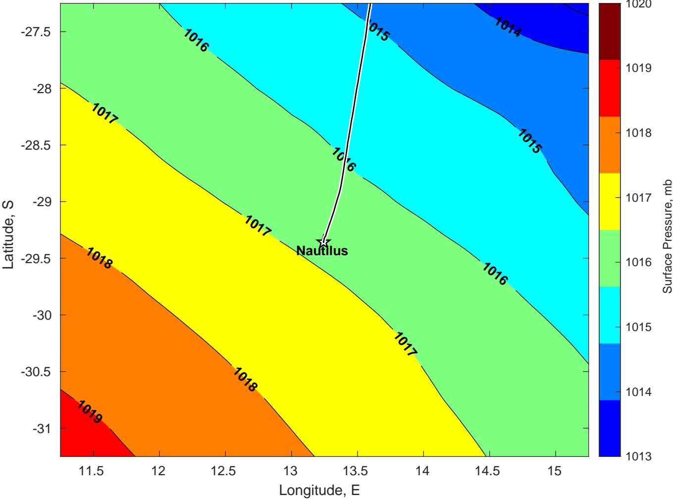
Surface Pressure (mb) for Nautilus at 24-Feb-2025 00:00:00
