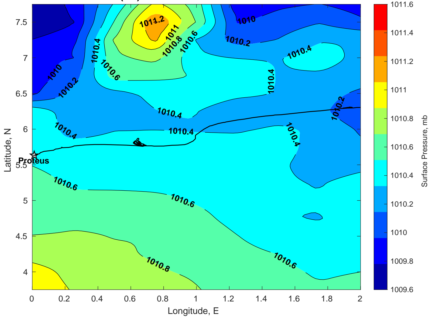
Surface Pressure (mb) for Proteus at 24-Feb-2025 00:00:00
