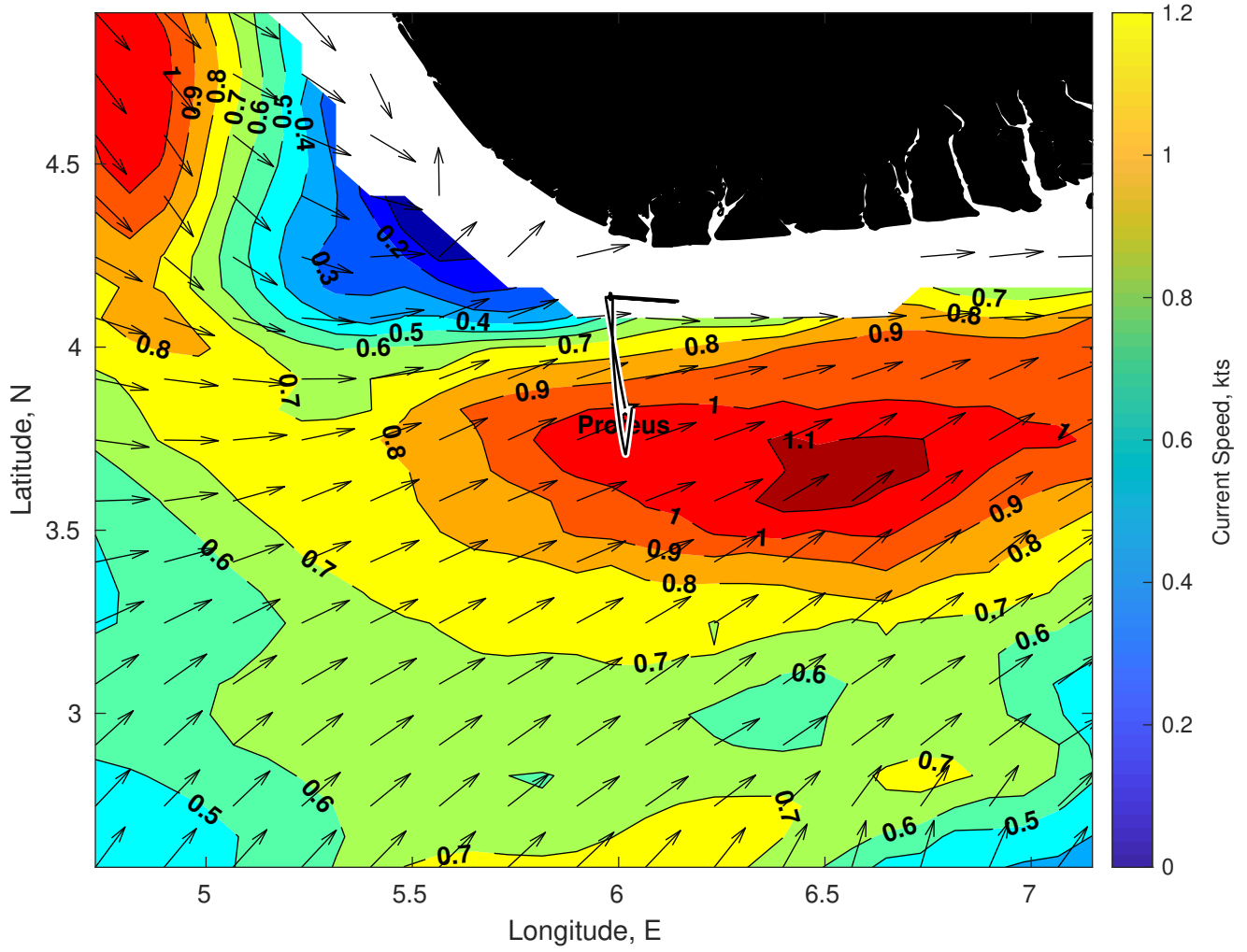
Surface Currents for Proteus at 21-Feb-2025 00:00:00
