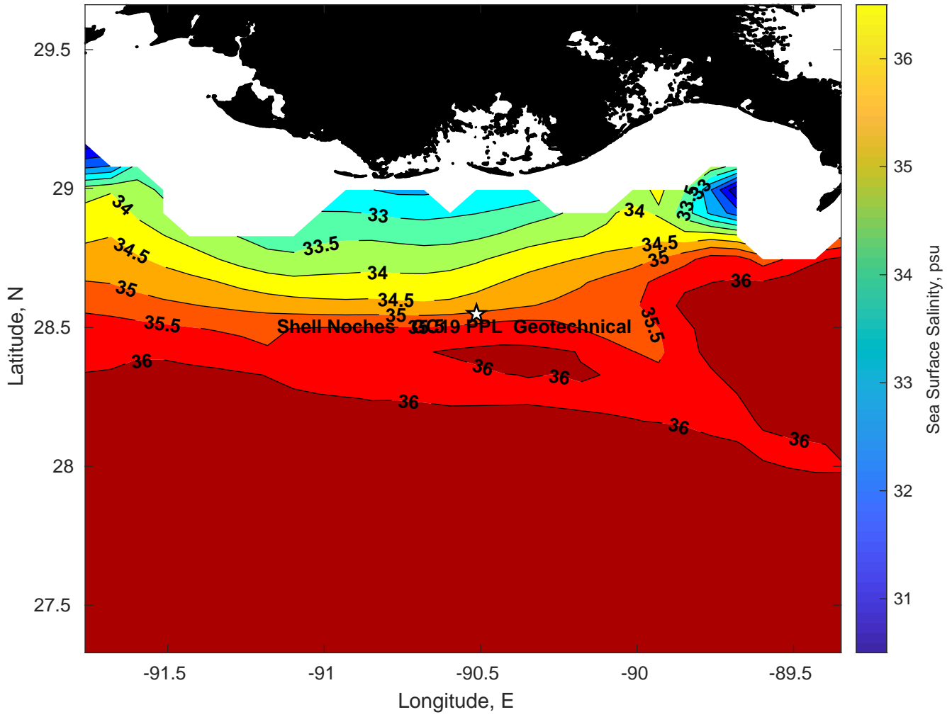
Surface Salinity for Shell Noches GC19 PPL Geotechnical at 21-Feb-2025 00:00:00
