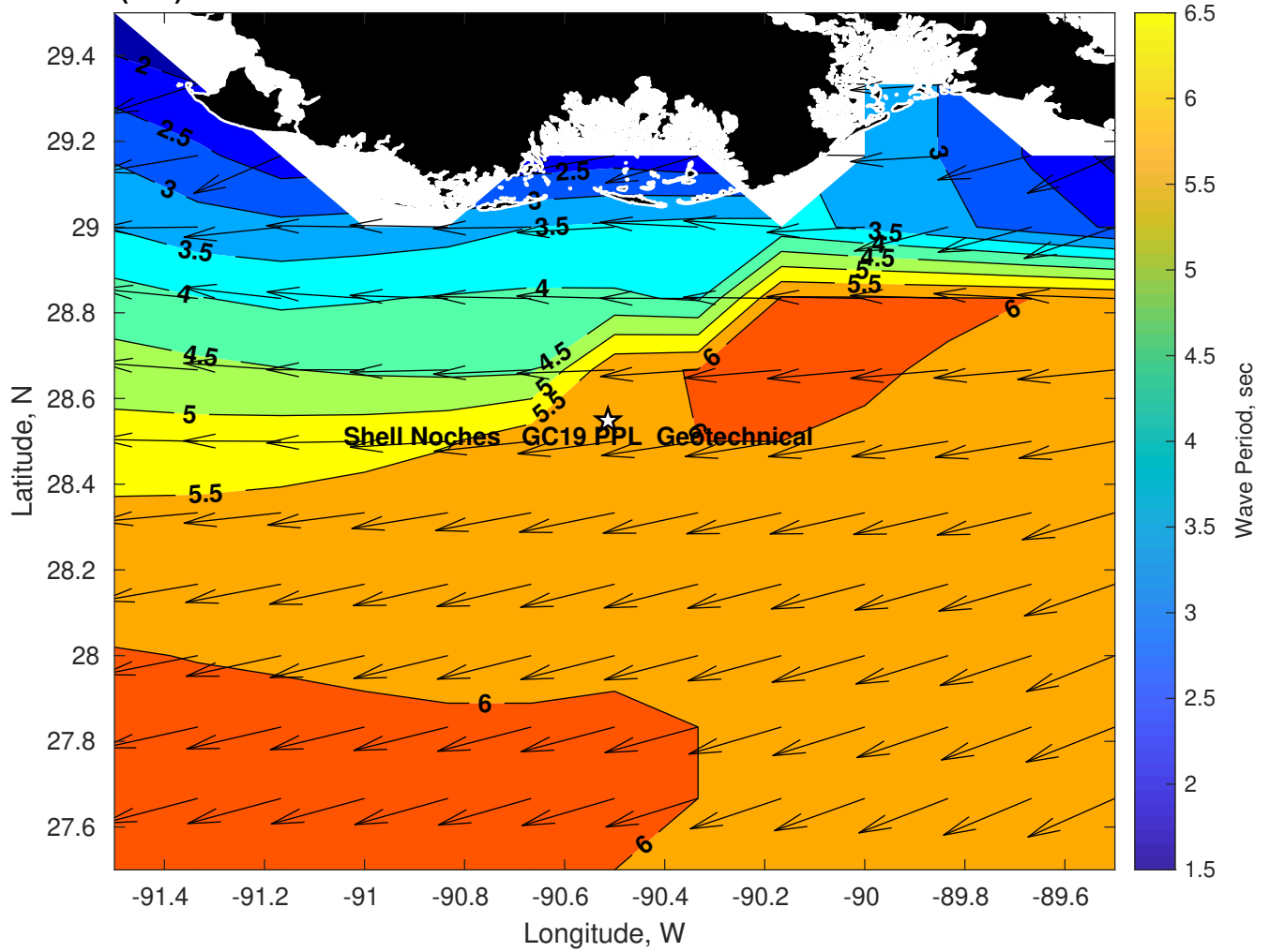
Wave Period (sec) for Shell Noches GC19 PPL Geotechnical at 22-Feb-2025 09:00:00
