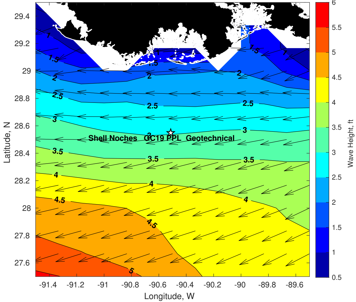
Wave Height (ft) for Shell Noches GC19 PPL Geotechnical at 22-Feb-2025 09:00:00
