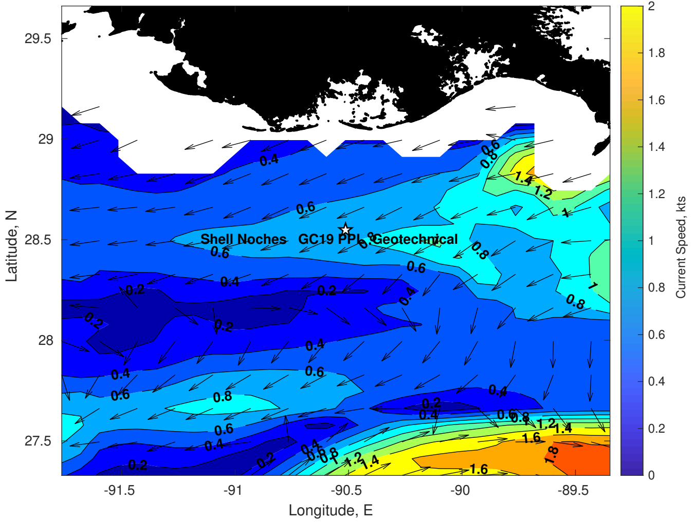
Surface Currents for Shell Noches GC19 PPL Geotechnical at 21-Feb-2025 00:00:00
