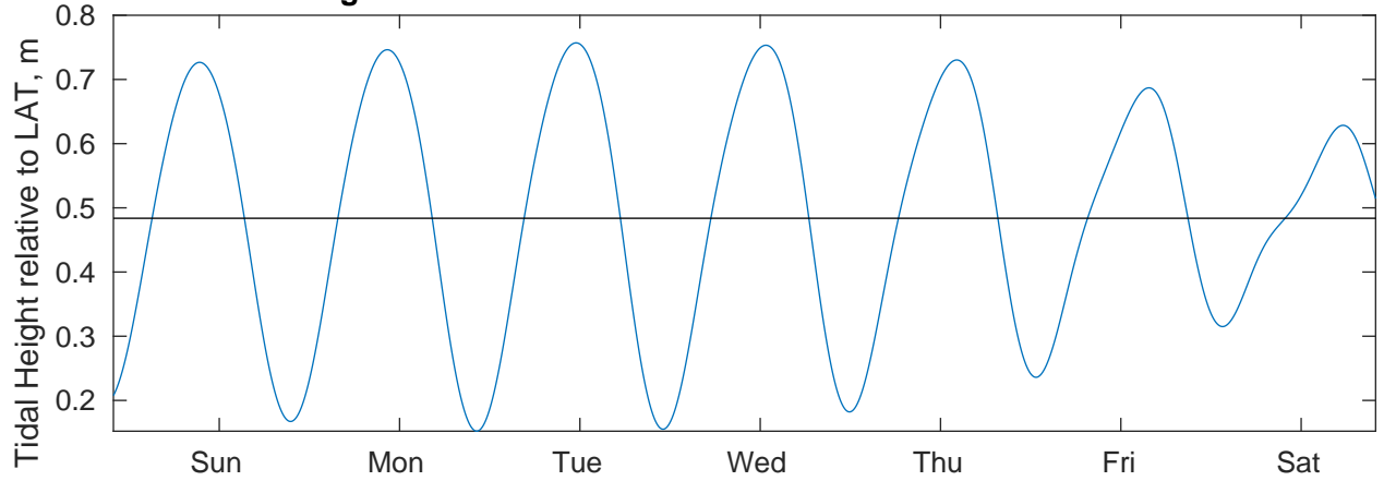
Tidal Currents and Heights for Shell Noches GC19 PPL Geotechnical at 20250222
