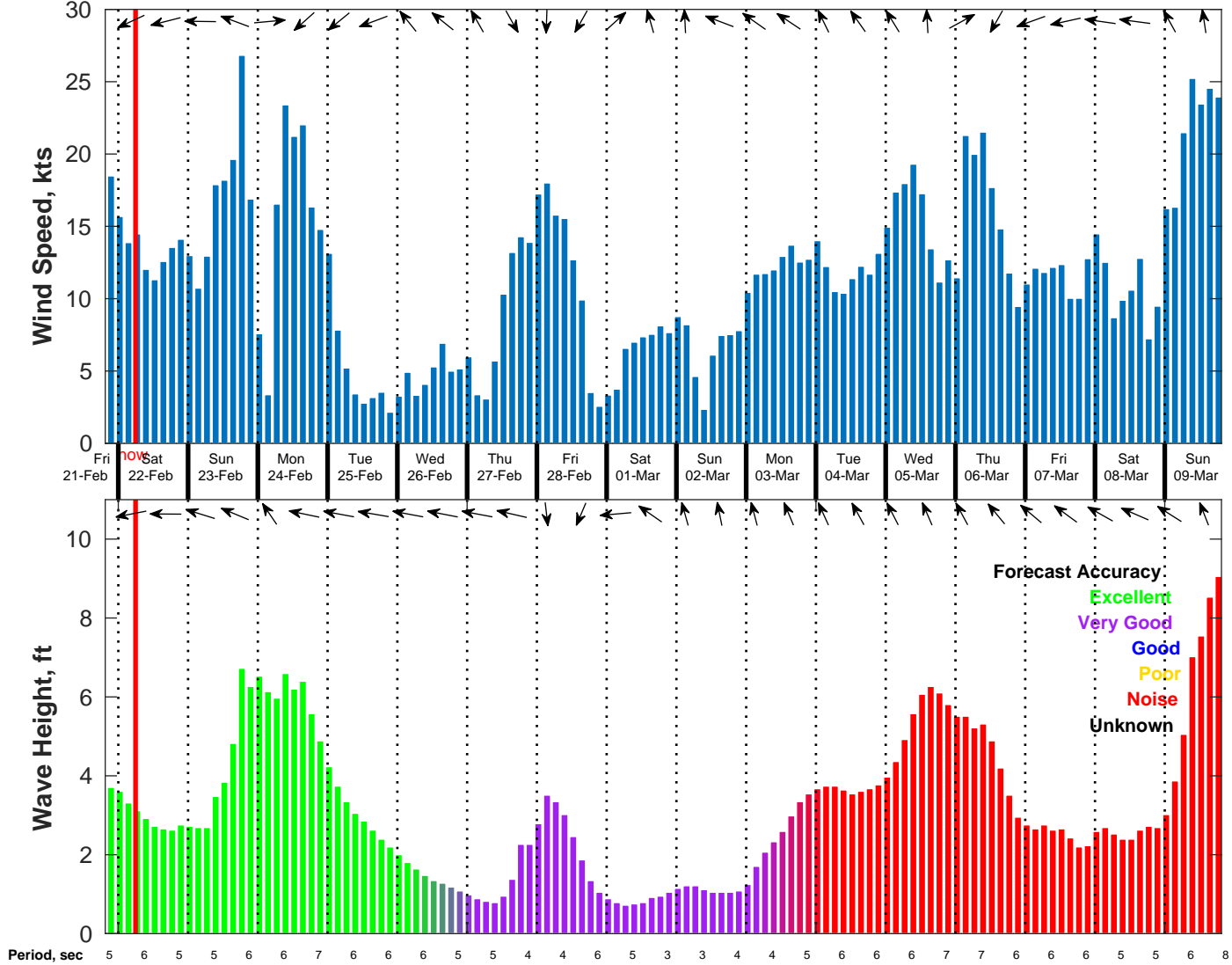
Wind & Wave Forecast for Shell Noches GC19 PPL Geotechnical from 21-Feb-2025 20:00:00 to 09-Mar-2025 20:00:00
