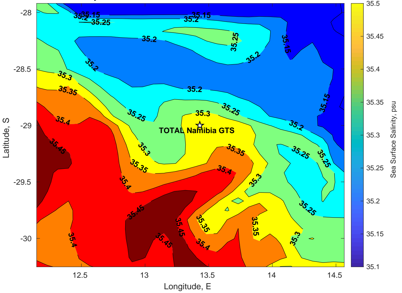
Surface Salinity for TOTAL Namibia GTS at 21-Feb-2025 00:00:00
