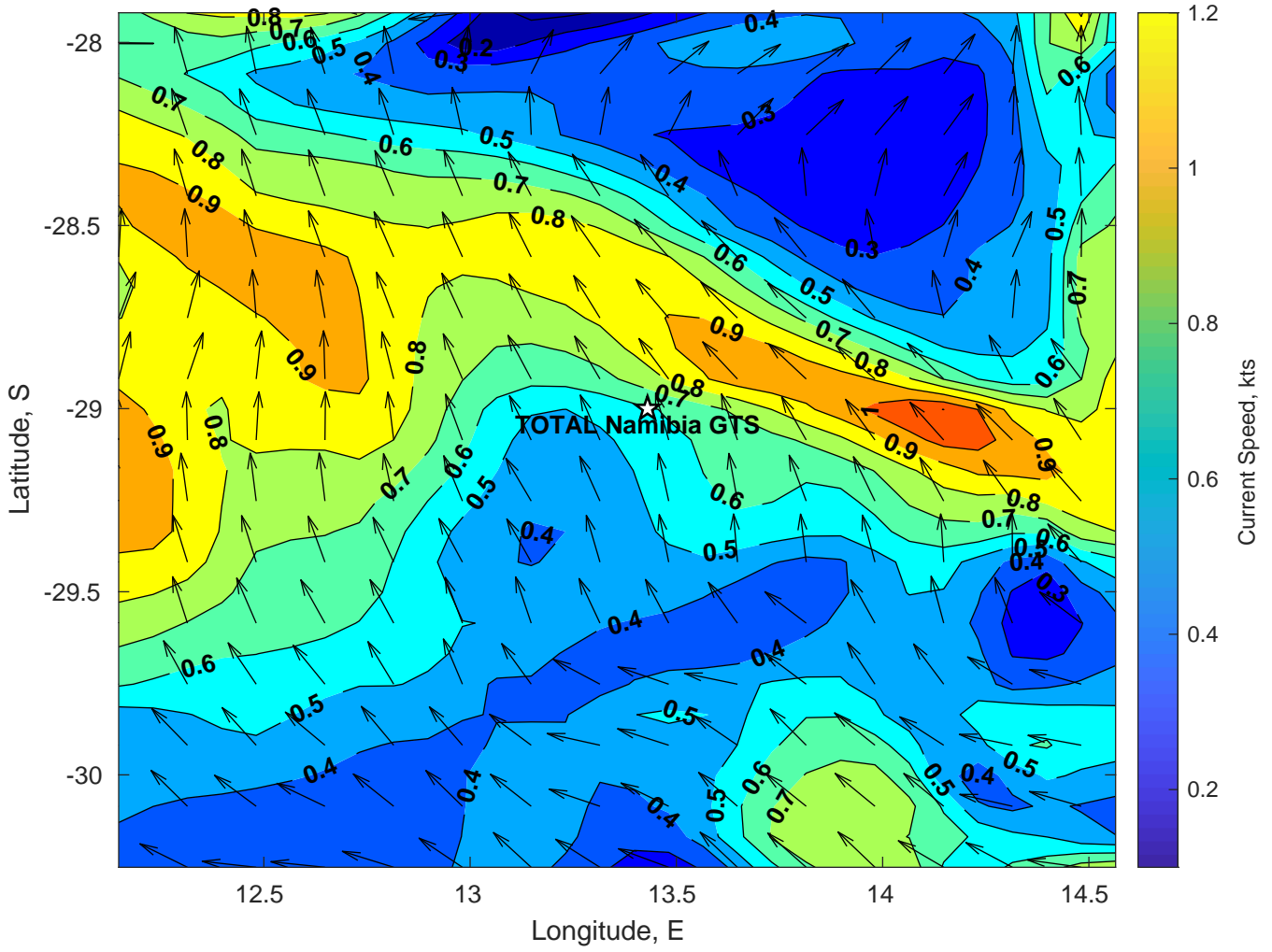
Surface Currents for TOTAL Namibia GTS at 21-Feb-2025 00:00:00
