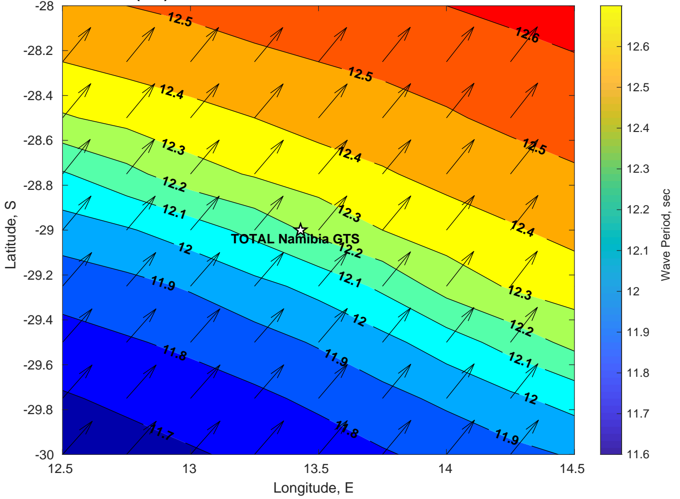
Wave Period (sec) for TOTAL Namibia GTS at 22-Feb-2025 09:00:00
