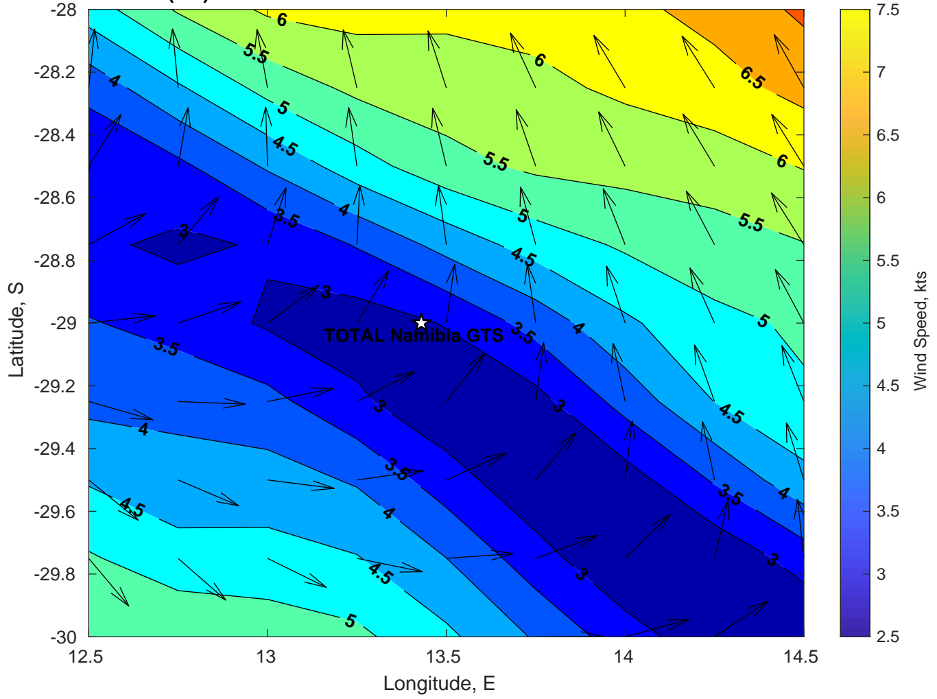
Winds (kts) for TOTAL Namibia GTS at 22-Feb-2025 09:00:00
