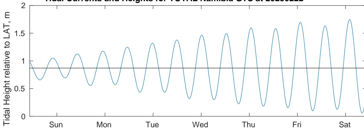
Tidal Currents and Heights for TOTAL Namibia GTS at 20250222
