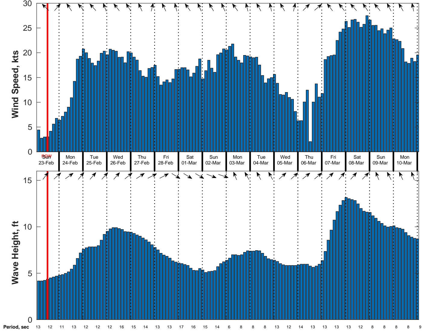
Wind & Wave Forecast for TOTAL Namibia GTS from 22-Feb-2025 02:00:00 to 10-Mar-2025 02:00:00
