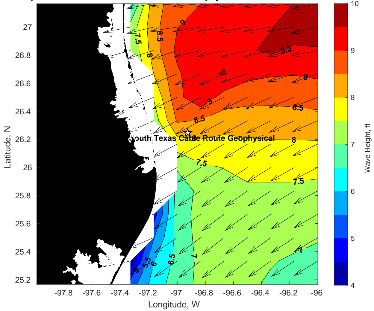
Wave Height (ft) for Tampnet P2378 South Texas Cable Route Geophysical at 22-Feb-2025 09:00:00
