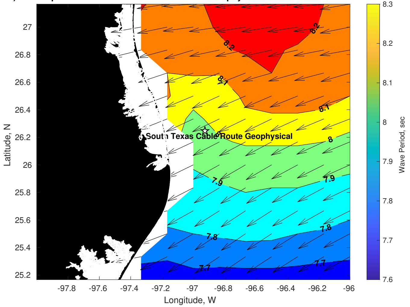
Period (sec) for Tampnet P2378 South Texas Cable Route Geophysical at 22-Feb-2025 09:00:00
