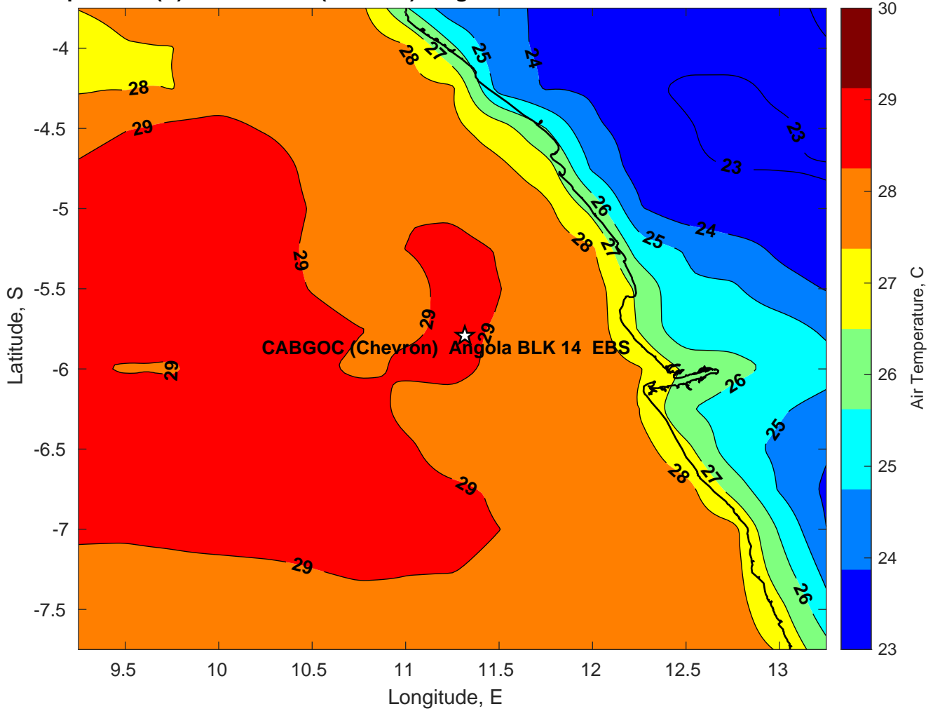
Air Temperature (C) for CABGOC (Chevron) Angola BLK 14 EBS at 23-Feb-2025
