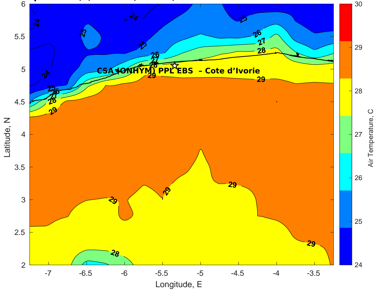
Air Temperature (C) for CSA (ONHYM) PPL EBS - Cote d'Ivoire at 23-Feb-2025
