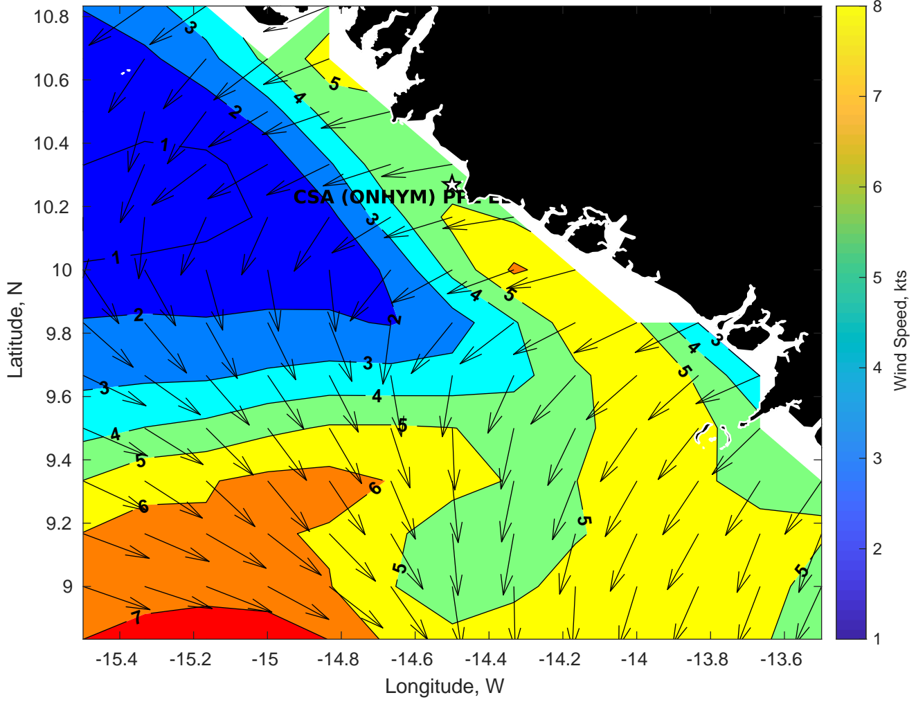
Winds (kts) for CSA (ONHYM) PPL EBS - Guinea at 23-Feb-2025 09:00:00
