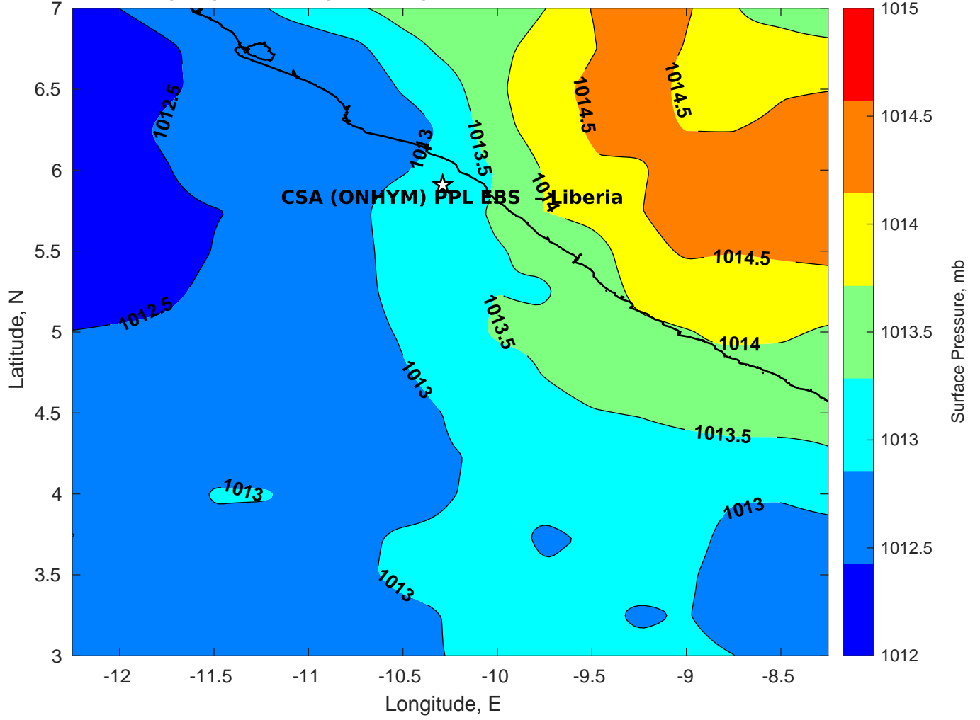
Surface Pressure (mb) for CSA (ONHYM) PPL EBS - Liberia at 24-Feb-2025 00:00:00
