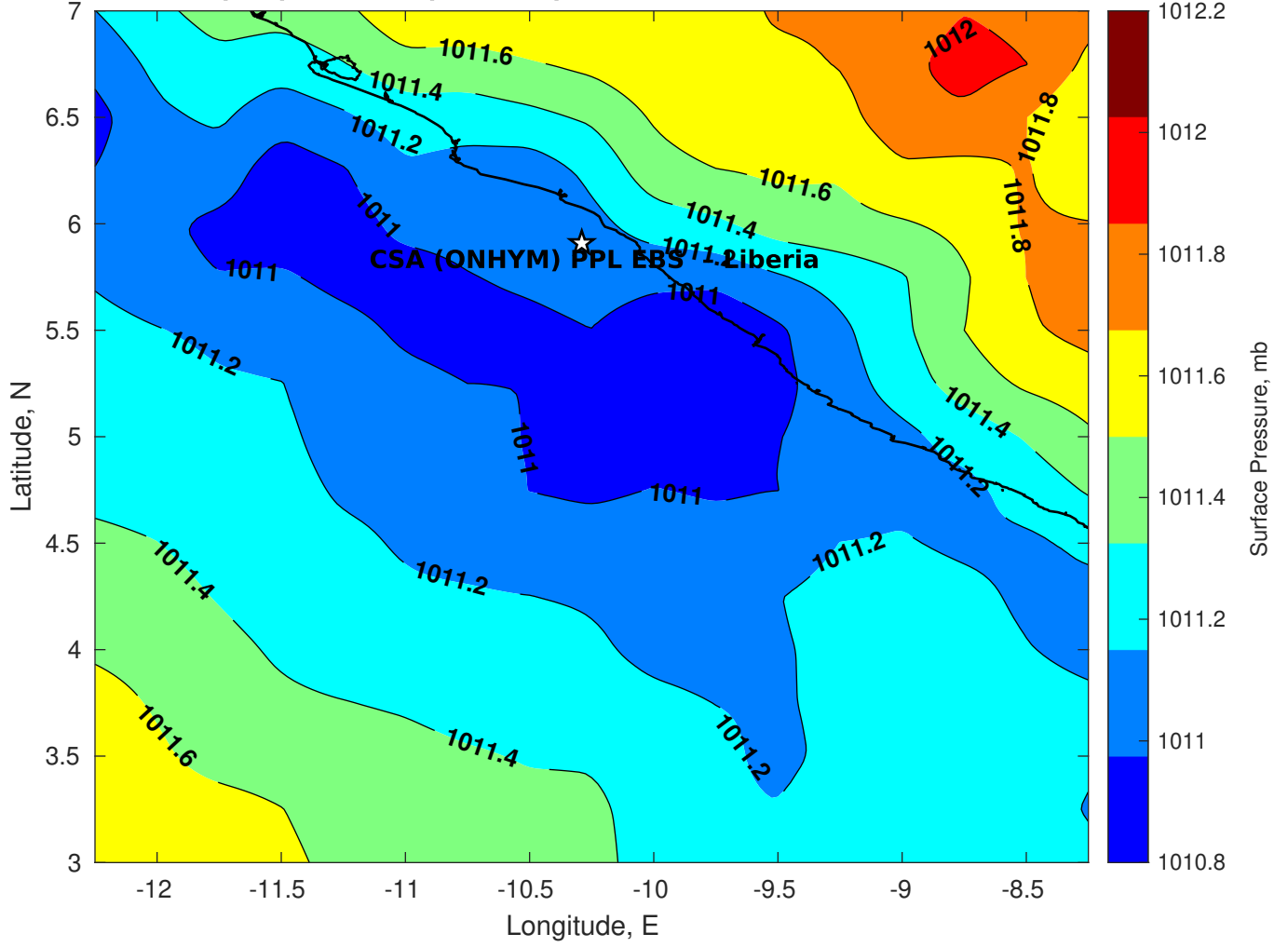
Surface Pressure (mb) for CSA (ONHYM) PPL EBS - Liberia at 23-Feb-2025 00:00:00
