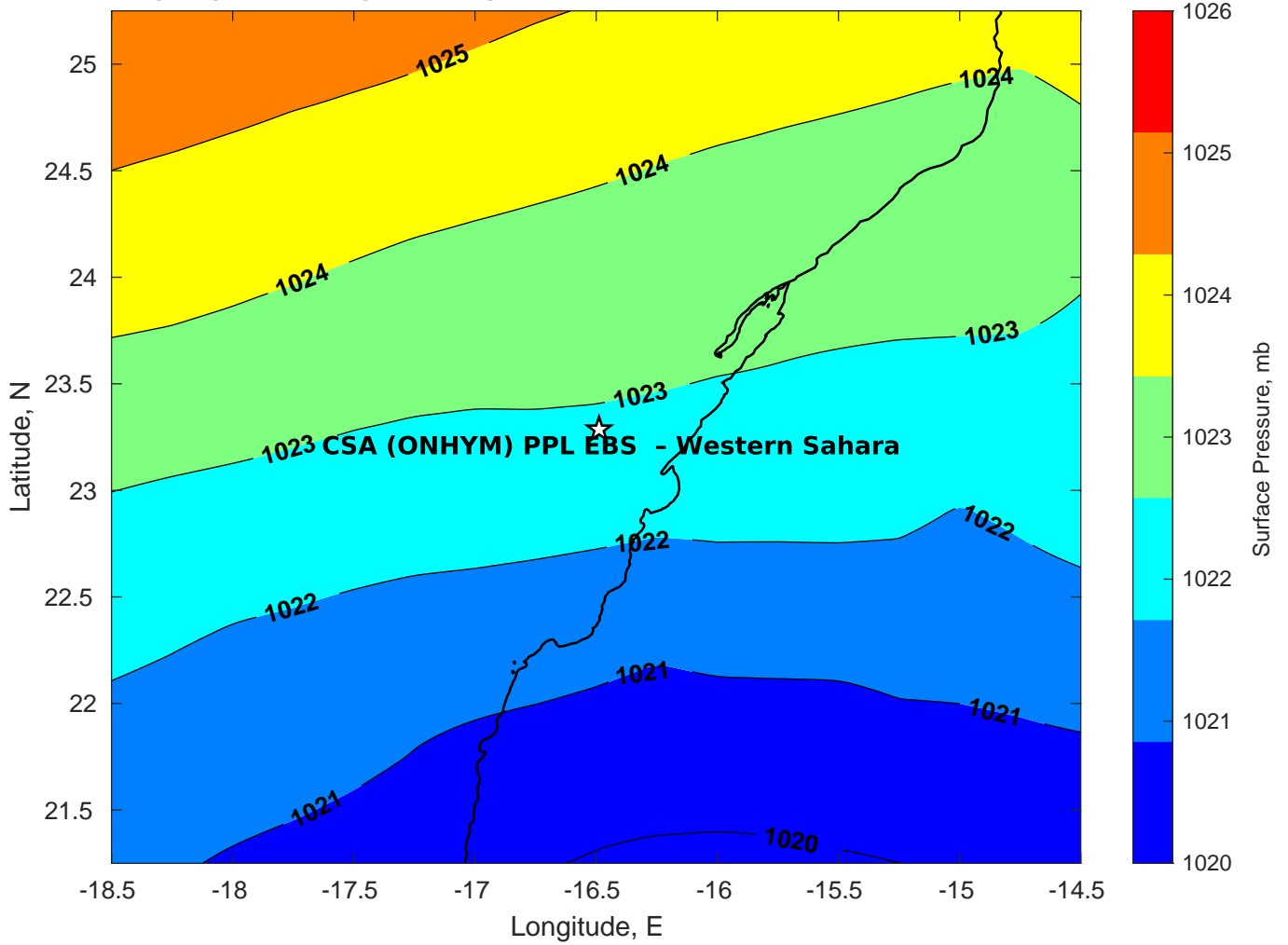
Surface Pressure (mb) for CSA (ONHYM) PPL EBS - Western Sahara at 25-Feb-2025 00:00:00
