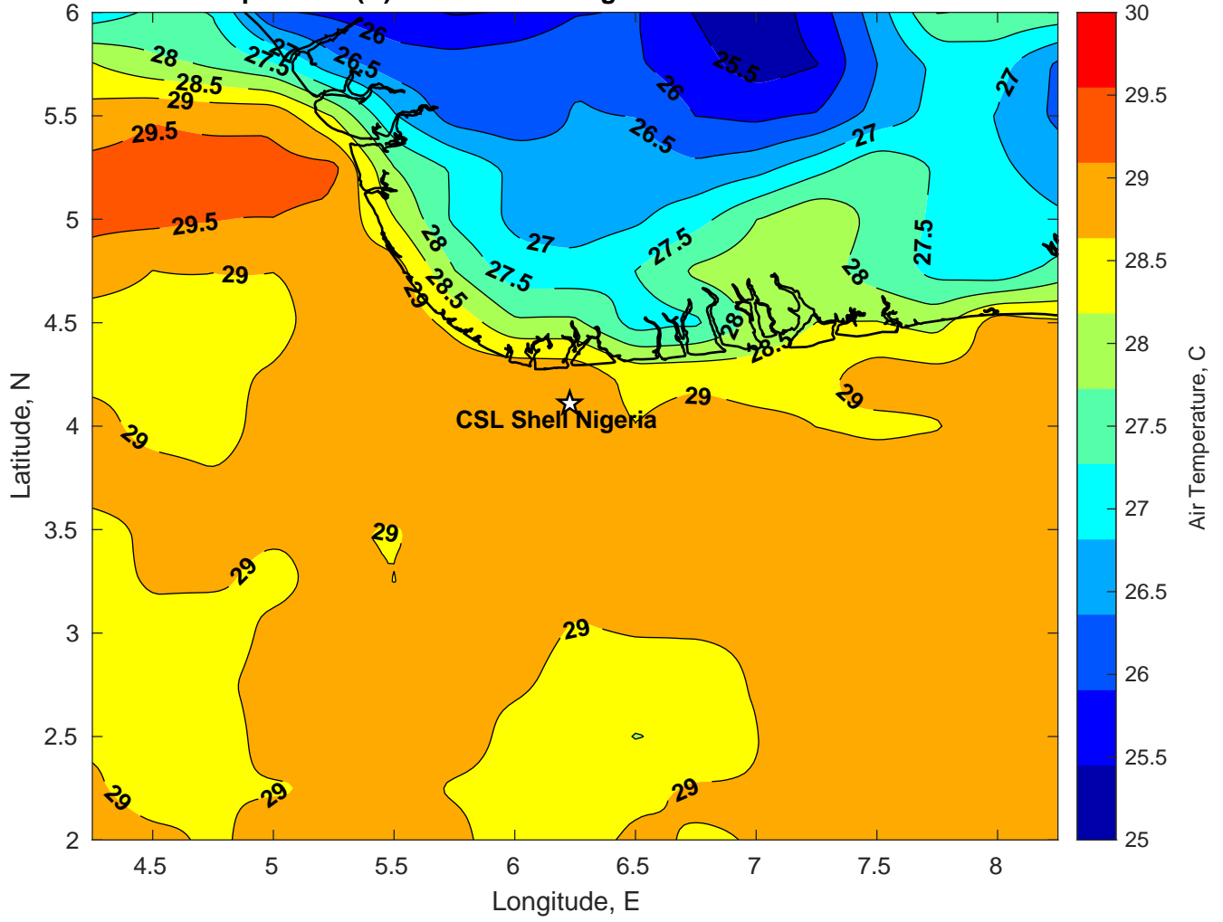
Air Temperature (C) for CSL Shell Nigeria at 23-Feb-2025
