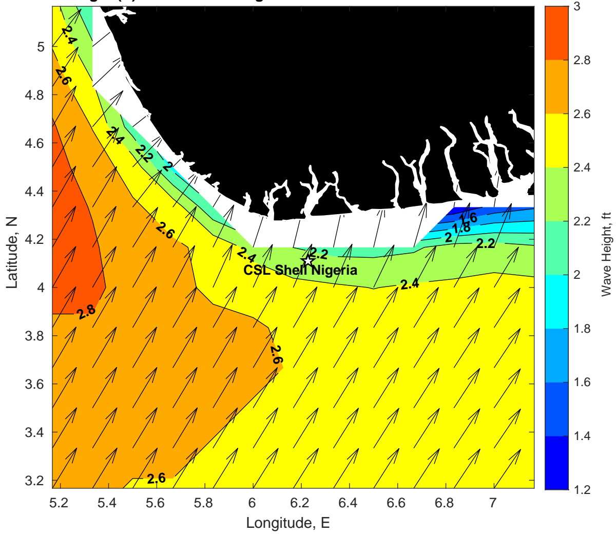
Wave Height (ft) for CSL Shell Nigeria at 23-Feb-2025 09:00:00
