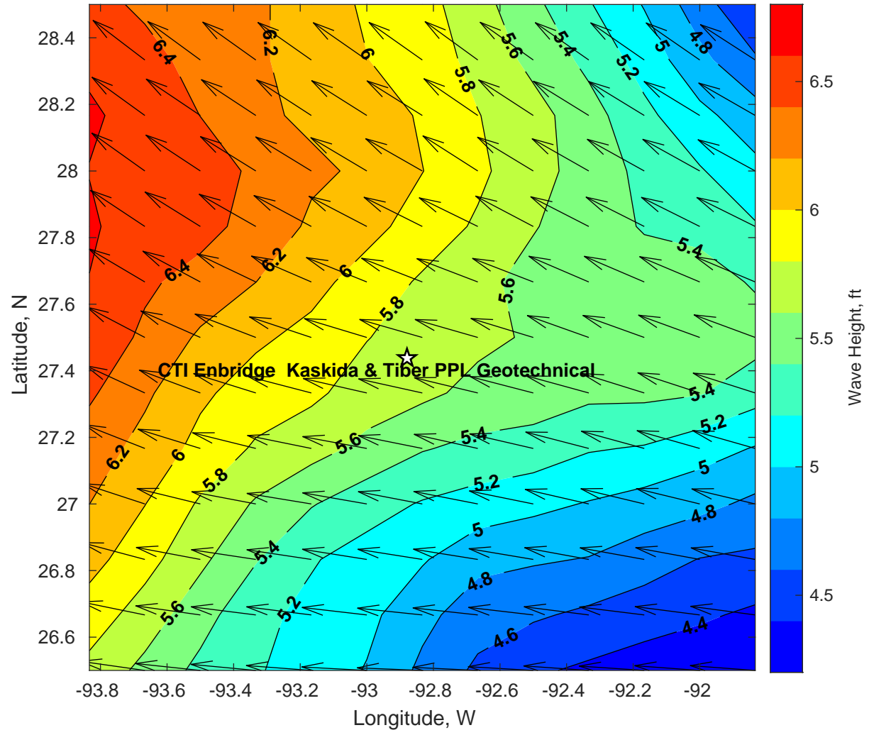
Wave Height (ft) for CTI Enbridge Kaskida & Tiber PPL Geotechnical at 23-Feb-2025 09:00:00
