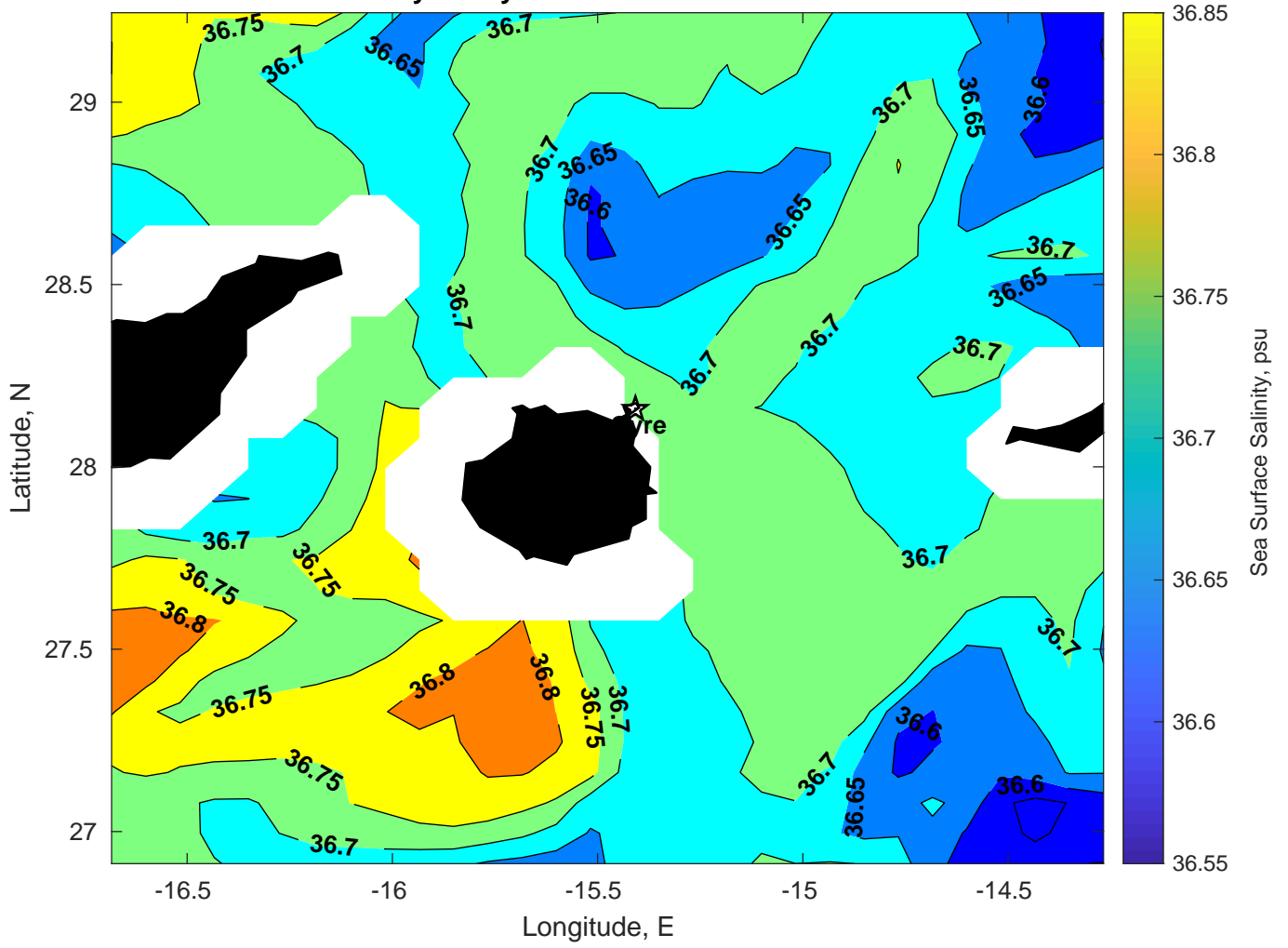
Surface Salinity for Gyre at 22-Feb-2025 00:00:00
