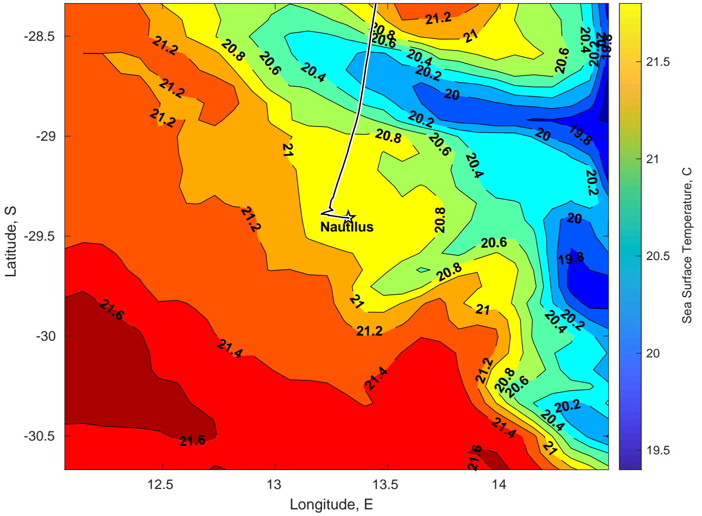
SST for Nautilus at 22-Feb-2025 00:00:00
