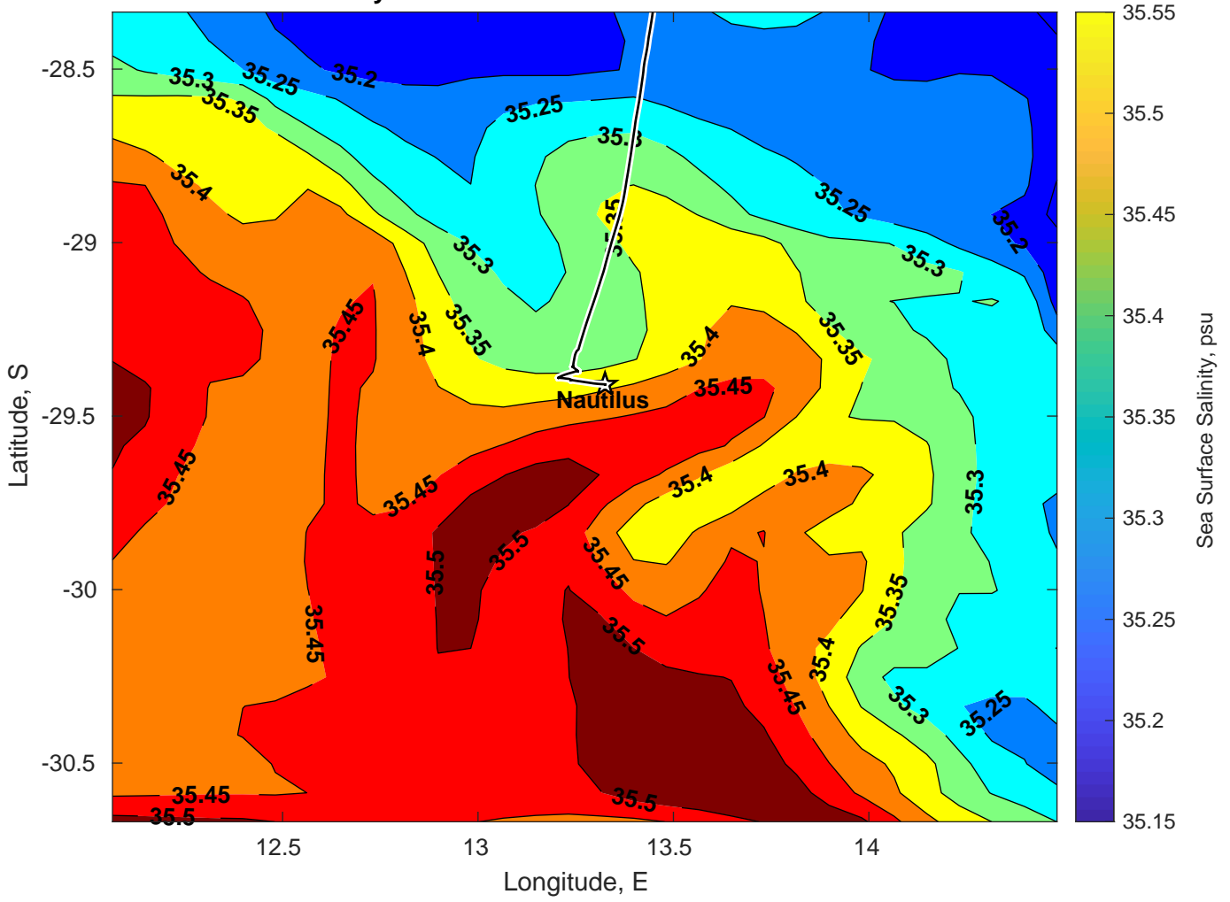
Surface Salinity for Nautilus at 22-Feb-2025 00:00:00
